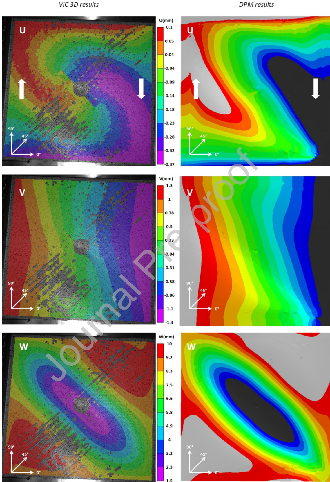
Figure 16: Experimental and DPM displacement fields in shear just before failure
