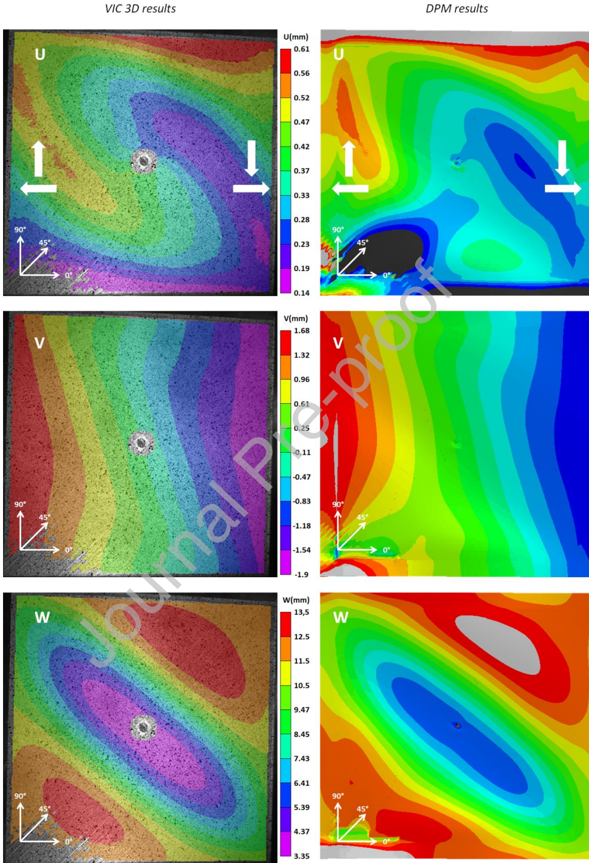
Figure 24: Experimental and DPM displacement fields in tension/shear just before failure
