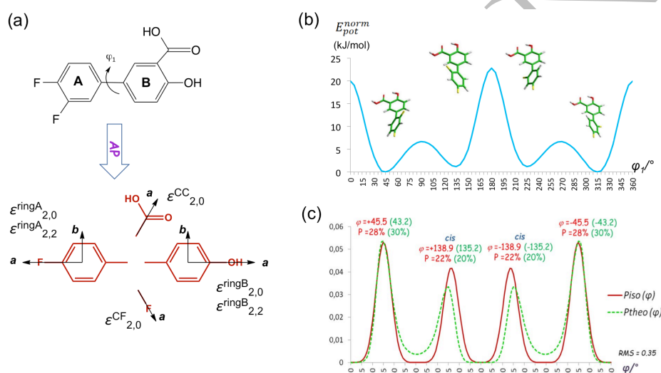
Figure 50 (a) AP modelisation of U_{ext}(\Omega, \{\phi\}) applied to diflusal. (b) Variation of normalized potential energy as a function of \varphi_1 obtained from B3LYP/6-31++G** calculations in vacuo. (c) Modelisation of P_{iso}(\varphi) of DFL compared to its in vacuo theoretical torsional curve P_{theo}(\varphi) . Figure adapted from Ref. [230] with permission.
