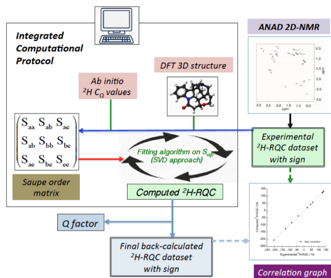
Figure 35 (a) Molecular structure and numbering of FCH. (b) Simplified flowchart showing the principle of molecular structural analysis using the integrated computational program “MSpin-RQC” from the ^2\text{H} -RQCs extracted from ANAD 2D-NMR experiments. The correlation plot ( ^2\text{H-RQC}^{\text{Calc.}} vs. ^2\text{H-RQC}^{\text{Exptl.}} ) simply visualizes the quality of fit of experimental data. Figure from Refs. [2] with permission.
