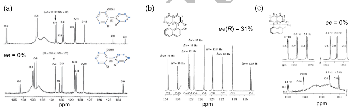
Figure 21 Four examples of atypical chirality (atropoisomerism) revealed by ^{13}\text{C} - \{^1\text{H}\} NMR (100.3 MHz) in the PBLG mesophase. Figure adapted from Refs. [20], [21] and [28] with permission.
