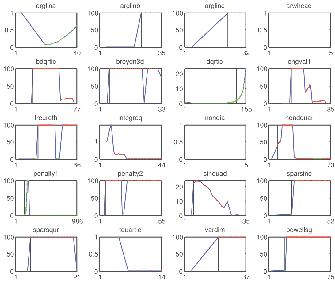
Fig. 2. Plots of the indicator values I_k/I_{\text{scaling}} in the hybrid I^1/I^2 case when they were calculated (points, in green or lighter for I_k^1 and in red or darker for I_k^2 ). The solid (blue) line is plotted for better visualization. The (black) vertical line signals the moment of the switch. Note that in the x -axis we count iterations, not function evaluations, and that all indicator values above 100 were plotted using this value for better visualization. (For interpretation of the references to colour in this figure legend, the reader is referred to the web version of this article.)
