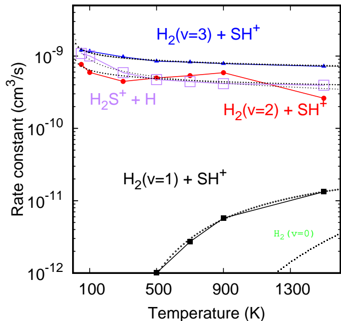
Fig. A.1. Calculated rate constants as a function of temperature (for translation and rotation) for SH + ( v=0, j=0 ) + H 2 ( v=1, 2, 3, j=0 ) and H 2 S + ( v=0, j=0 ) + H reactions (lavender) using ZPE corrected QCT method. Dotted curves are fits of the form k(T) = \alpha (T/300)^\beta \exp(-\gamma/T) . Rate coefficients are listed in Table 1.
