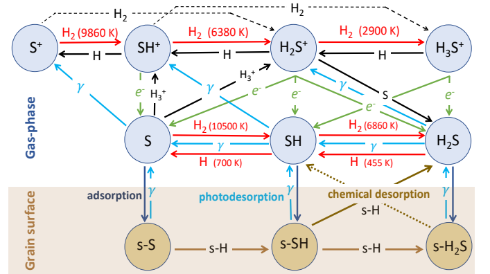
Fig. 11. Main gas and grain reactions leading to the formation of sulfur hydrides. Red arrows represent endoergic reactions (endothermicity given in units of K). Dashed arrows are uncertain radiative associations (see Appendix A.3), \gamma stands for a FUV photon, and “s-” for solid.
