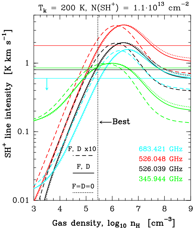
Fig. 6. Non-LTE excitation models of \text{SH}^+ . The horizontal lines mark the observed line intensities in the Orion Bar. Dotted curves are for a standard model ( F=D=0 ). Continuous curves are for a model that includes chemical destruction by H atoms and e^- (model F, D ). Dashed lines are for a model in which destruction rates are multiplied by ten (model F, D \times 10 ). The vertical black line marks the best model.
