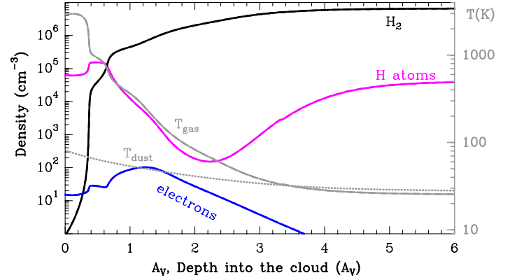
Fig. 10. Structure of an isobaric PDR representing the most FUV-irradiated gas layers of the Orion Bar (see Table 2 for the adopted parameters). This plot shows the \text{H}_2 , H, and electron density profiles (left axis scale), and the gas and dust temperatures (right axis scale).
