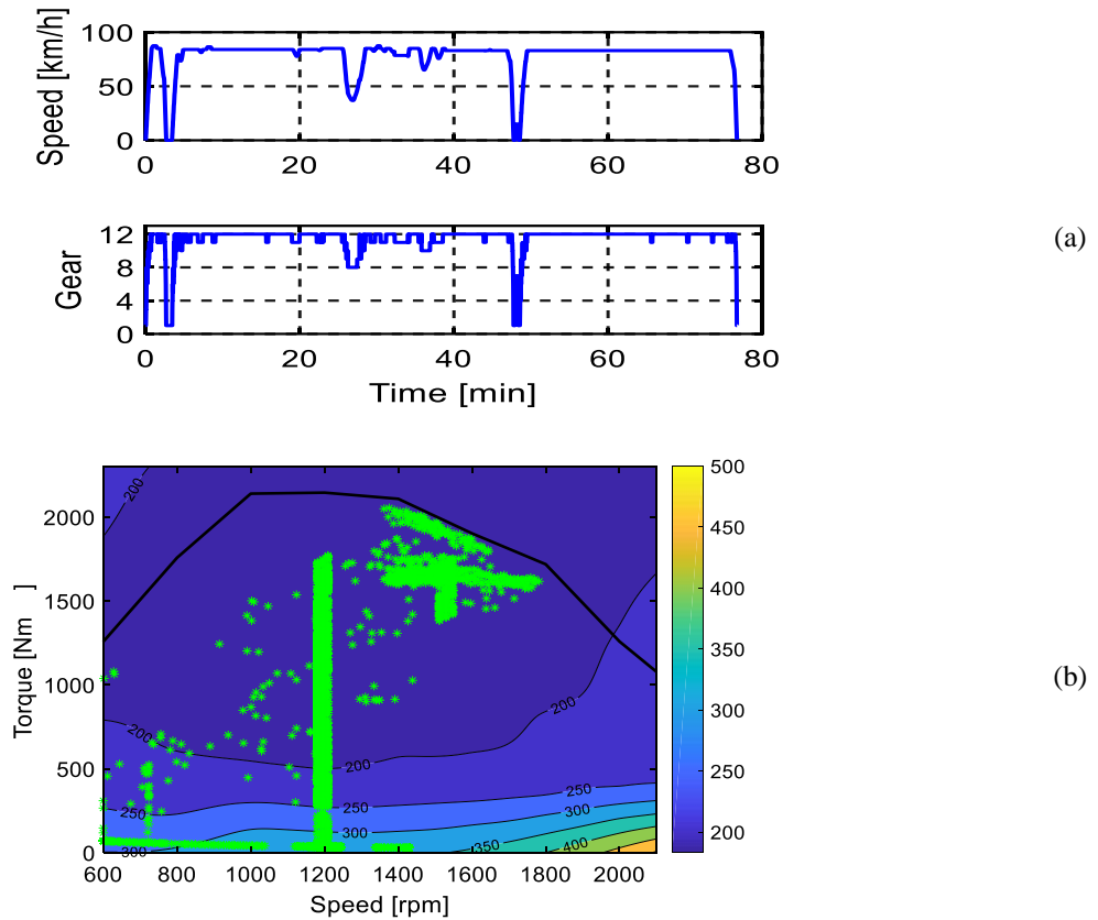
Fig. 4: Dynamic programming results for the reference truck: (a) Gear shifting result, (b) Engine operating points: Brake specific fuel consumption [g/kWh] as a function of engine speed and torque
