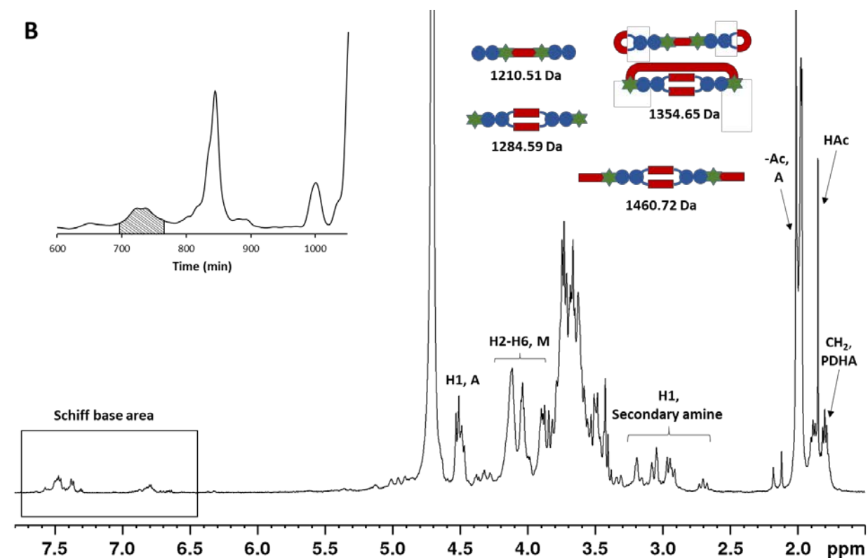
Figure S5: 1 H-NMR characterisation of fraction B from Figure S3. The structures identified by MS are included in the figure.
