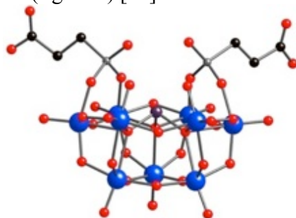
Fig. 1: Structural representation of the bis-propanoic acid phosphonyl derivative [\text{As}^{\text{III}}\text{W}_9\text{O}_{33}\{\text{P}(\text{O})(\text{CH}_2\text{CH}_2\text{CO}_2\text{H})\}_2]^{2-} anion. The W, As, P, O and C atoms are shown respectively in blue, prune, grey, red and black.
