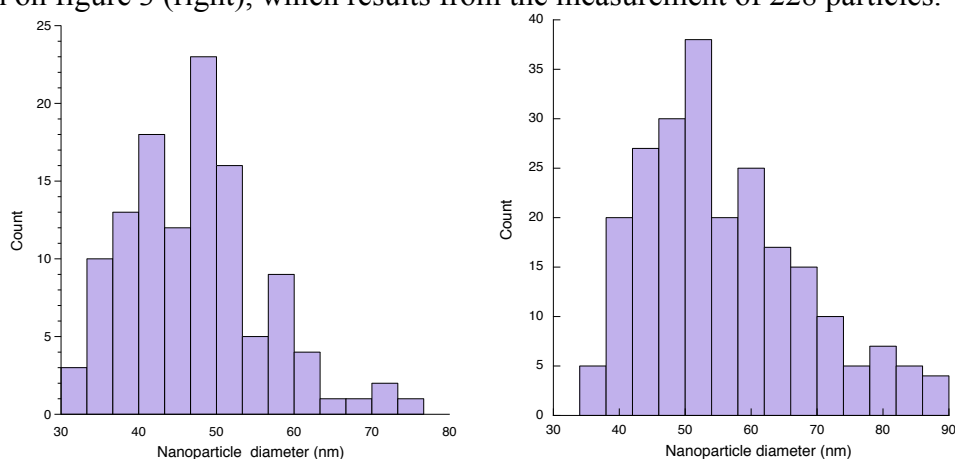
Fig. 3: Size histograms for POM-CO 2 H-decorated MNPs sample with (left) unsorted and (right) sorted (9 nm) maghemite cores, counted from TEM micrographs.
