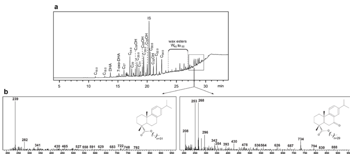
Figure 5: Example of TLE containing unusual molecular compounds eluted after the wax esters (sample LD10662a). a) partial gas chromatogram; b) mass spectra of the peaks eluted at 28 min and proposed molecular structures.
