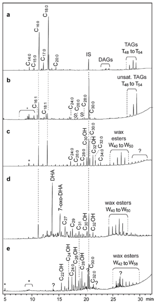
Figure 2: Gas chromatograms of lipids from ceramic vessels (a to d) and of sediment (e). a) animal fat (LD10676a); b) plant oil (MR2707r); c) plant wax (LD10669a); d) beeswax and conifer resin (LD10662a). C_{xx} : fatty acids; DHA: dehydroabietic acid; C_{xx}OH : linear alcohols; C_{xx} : linear alkanes; S: saccharides; DAGs: diacylglycerols; W_{xx} : wax esters; TAGs: triacylglycerols; ?: unknown compound; IS: internal standard; *: modern contamination.
