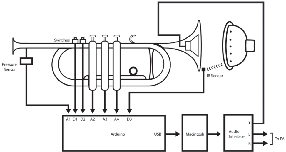
Figure 6. !trumpet system.
