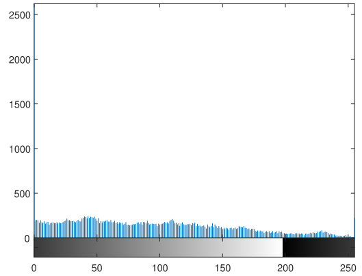
FIGURE 11. Histogram of Lena selective encrypted image with size of 256 x 256.
