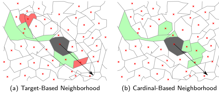
Figure 2: Toy example of path-based neighborhoods. The arrow indicates the orientation of \mathbf{g}_s and superpixels of neighborhood are shown in color. For TBN, two “targets” (in red) are selected in an ellipse centered on the source superpixel s (in grey). For CBN, two paths with K = 3 elements are built to be aligned with \mathbf{g}_s , taking into account radiometric similarity with the site s .
