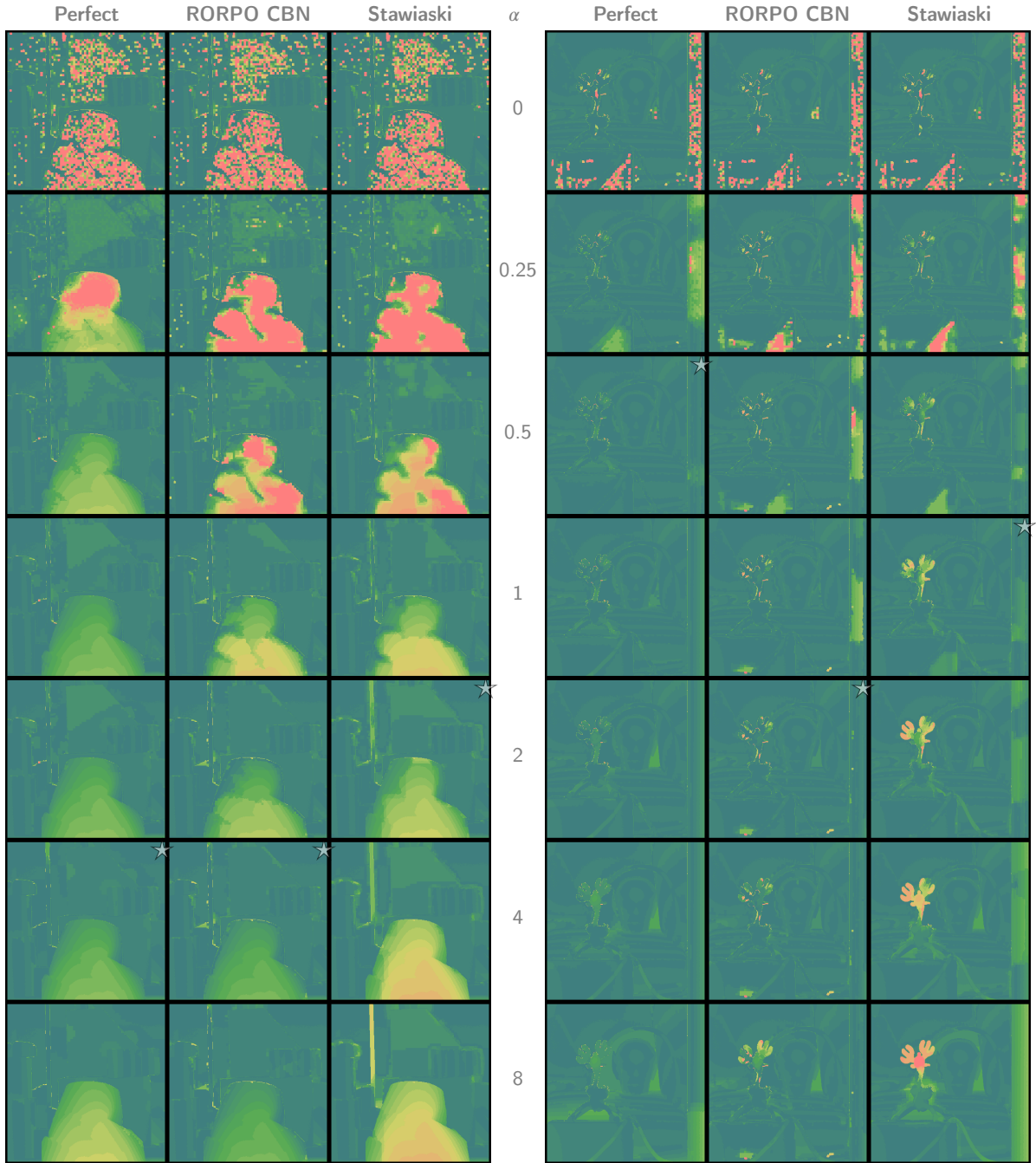
Figure 9: Maps of depth error obtained for the scenes Lampshade (left) and Reindeer (right), for three neighborhood construction strategies ( Perfect , RORPO CBN and Stawiaski) and different values of regularization parameter \alpha \in \{0., 0.25, 0.5, 1, 2, 4, 8\} . For better visualization, error value dynamic has been bounded to \frac{2\Delta h}{5} .
