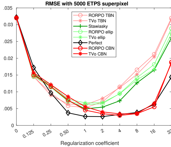
Figure 3: Comparison of neighborhood anisotropy benefit measured through RMSE (y-axis) on the whole dataset. The results are achieved using 5000 ETPS superpixels [29] and different neighborhood estimations.
