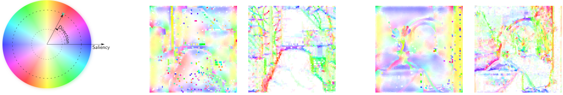
Figure 8: Comparison of guidance maps g for Lampshade and Reindeer scenes, using a color representation, such that the saturation and the hue encode respectively the saliency and the orientation; from left to right: Color wheel, TVo Lampshade , RORPO Lampshade , TVo Reindeer , RORPO Reindeer .
