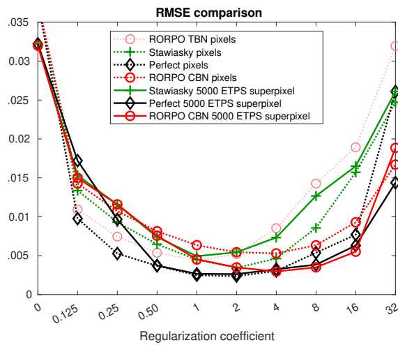
Figure 10: Superpixel versus pixel level: Comparison in terms of RMSE (y-axis) computed on the whole dataset, for three kinds of neighborhoods.
