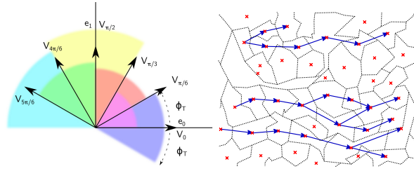
Figure 1: Illustration of the 6 directions of \mathcal{R} (left) and an example of path obtained with one structuring function \rightsquigarrow_\theta (right). The connectedness \rightsquigarrow_\theta is characterized by the vector \mathbf{v}_\theta and the angular width \phi_T . For this illustration, we have represented directed edges for positive displacements, but the paths are computed in both directions.
