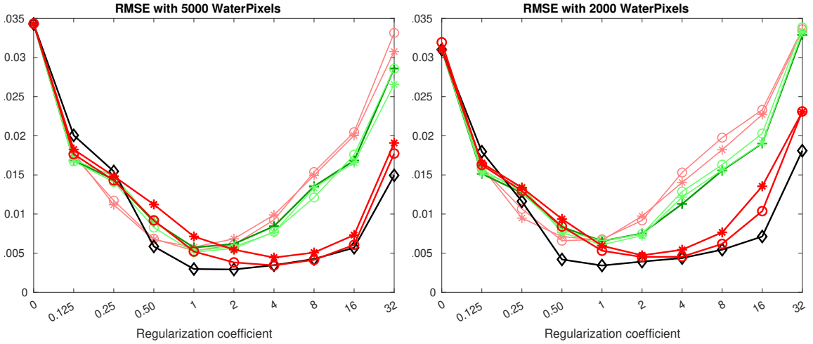
Figure 4: Comparison of neighborhood anisotropy benefit measured through RMSE (y-axis) on the whole dataset. The results are achieved using either 5000 WP (left) or 2000 WP (right) using different neighborhood estimations. The legend is the same as in Figure 3.
