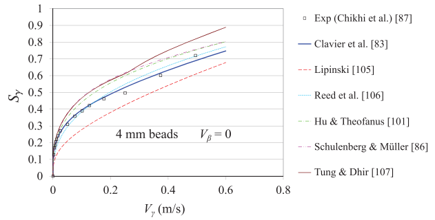
Figure 8. Experimental and modeling results for the gas saturation versus the gas velocity at V_\beta = 0 (from Clavier et al. in [104]).
