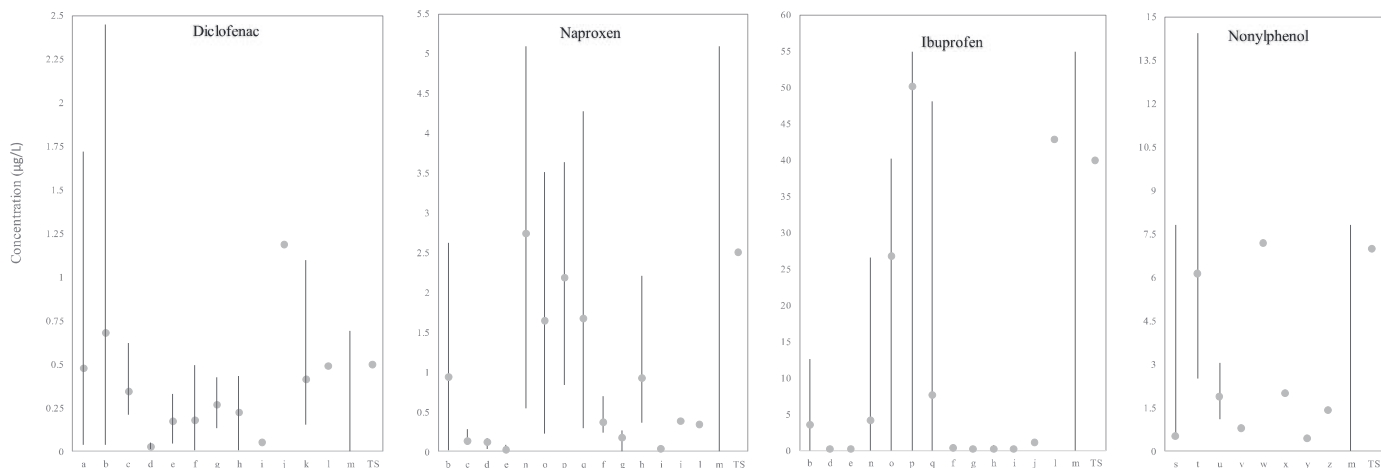
Fig. 2. Concentration range of target MPs in secondary-treated effluent of conventional wastewater treatment plants s found in literature (TS: This study, References: a [60], b [61], c [62], d [63], e [64], f-g [65], h [66], i [67], j [4], k [68], l [69], m [48], n-o-p-q [70], s [71], t-u [72], v [73], w [74], x [75], y [76], z [77]).
