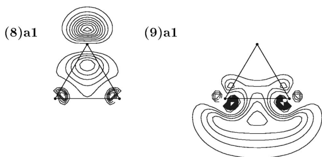
FIG. 2. Density contour plots of representative orbitals of Ag 2 Br.
