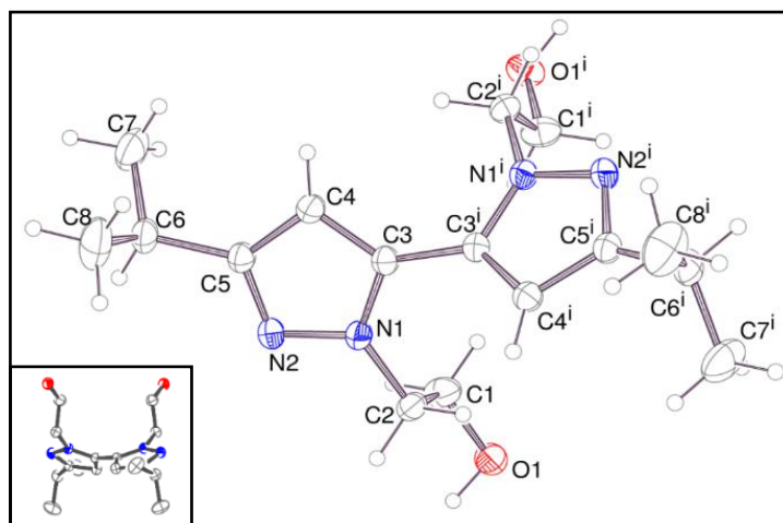
Figure 2. Representation of the C_{16}H_{26}N_4O_2 molecule with ellipsoids at 30% probability. The symmetry code used to generate equivalent atoms is i: x, -y, \frac{1}{2}-z . The view in ab plane (inset) makes clearer the molecule conformation.
