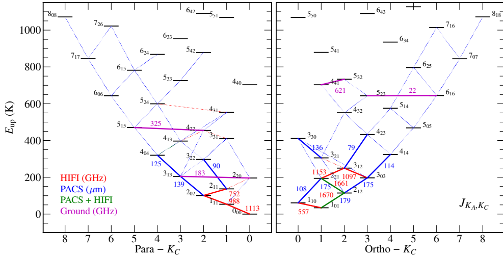
Fig. 1. Water rotational energy levels within the ground vibrational level. Transitions targeted with HIFI are indicated in red with frequencies in GHz, those with PACS in blue with wavelengths in \mu\text{m} . Dashed lines indicate water transitions detected in PACS and HIFI spectral scans. The 179 \mu\text{m} line observed with both PACS and HIFI is indicated in green. Purple lines indicate water (isotopolog) lines that can be observed from the ground with frequencies in GHz; some of them (e.g., 621 GHz) have also been observed with HIFI. The 22 GHz 6_{16}-5_{23} maser line observed at cm wavelengths is indicated.
