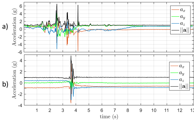
Fig. 2. 3D acceleration signals of two real falls of older adults: a) a fall captured using a wrist-worn device. b) a fall captured using a neck-worn device.
