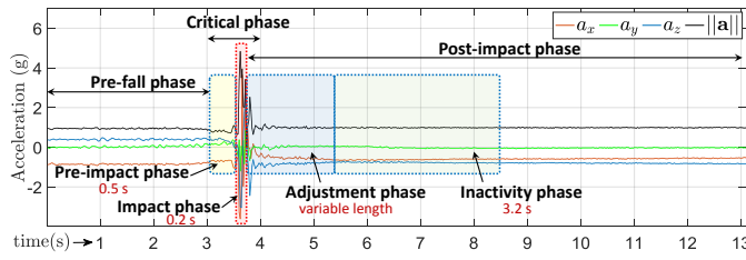
Fig. 7. Dynamic segmentation of a sliding window into different phases.
