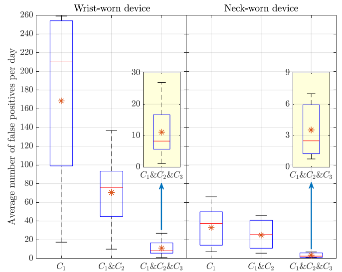
Fig. 3. The average number of false positives per day for wrist- and neck-worn devices represented in box plots. Results are first averaged per subject and then averaged per day.
