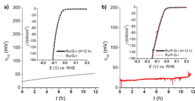
Figure 4. LSV of Ru/G-r (a) and Ru/P-G-r (b) before (dashed lines) and after (solid lines) a 12 h chronopotentiometry experiment at a j = -10 mA/cm². 26
