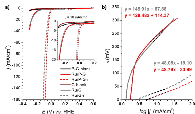
Figure 3. a) Polarization curves of Ru/G (grey line), Ru/P-G (red line) before (bold) and after (dashed) a reductive process at j = -10 mA/cm² in 1 M \text{H}_2\text{SO}_4 . G (wine line), P-G (black line) blanks are also shown. b) Tafel plots of Ru/G , Ru/G-r , Ru/P-G and Ru/P-G-r in 1 M \text{H}_2\text{SO}_4 . Same colour code as in (a).
