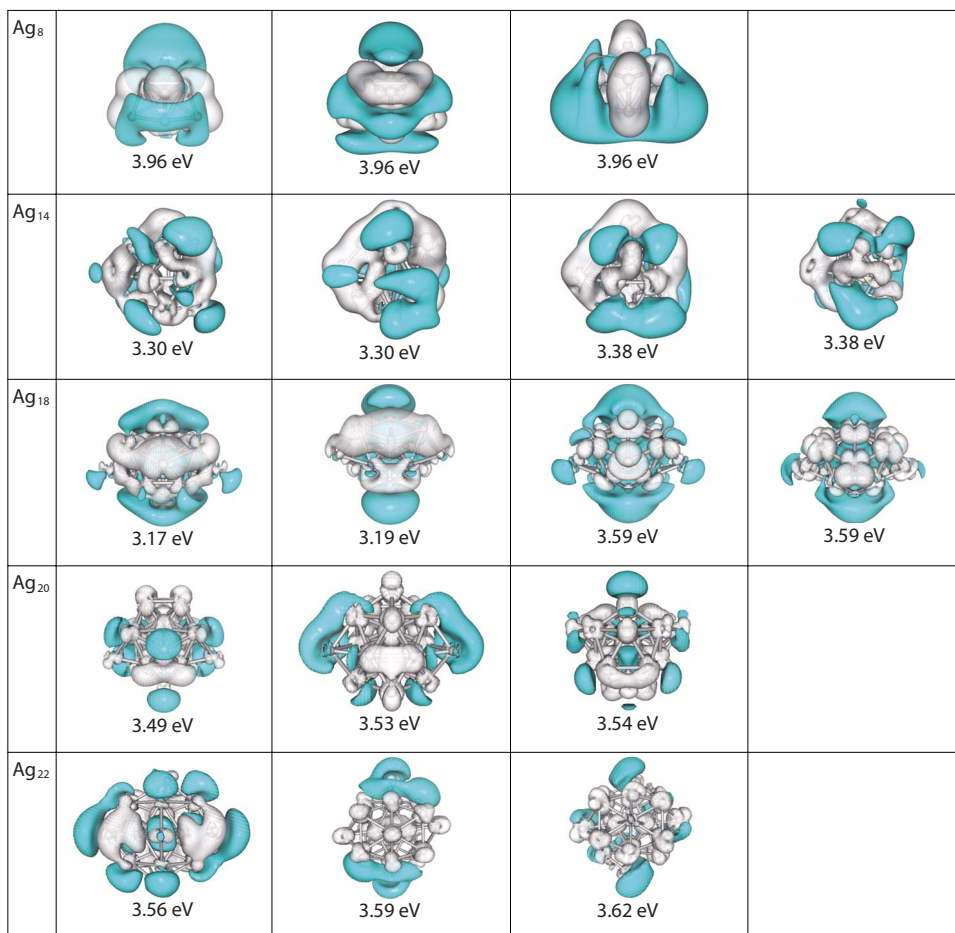
FIG. 6. (Color online) Electron density difference between the excited and the ground states for the main peaks in the cases of Ag 8 , Ag 14 , Ag 18 , Ag 20 , and Ag 22 clusters (isovalue of 0.0002 a.u.). Light regions correspond to the depletion of the electron density during the transition while blue (or dark) regions correspond to the accumulation. The transitions are due to the excitations from inner orbitals located on silver atoms to orbitals distributed on wide areas involving several atoms.
