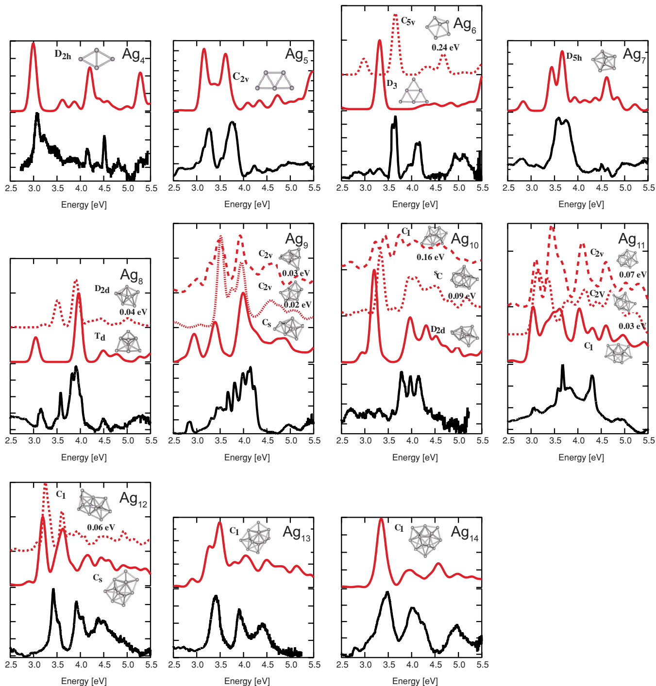
FIG. 1. (Color online) Absorption spectra of Ag_n , n=4-14 . Comparison between the experimental spectra (black line, bottom of each box) and the calculated ones for the lowest-energy isomers.
