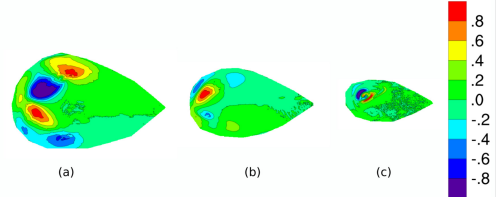
FIG. 7. Spatial distribution of mode 2 - (a) 2.3mm/s, (b) 3.3mm/s, (c) 4.3 mm/s
