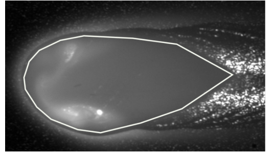
FIG. 3. Region of interest for a weld speed of 2.3mm/s after the calibration procedure; the image shows the view from below the plate.
