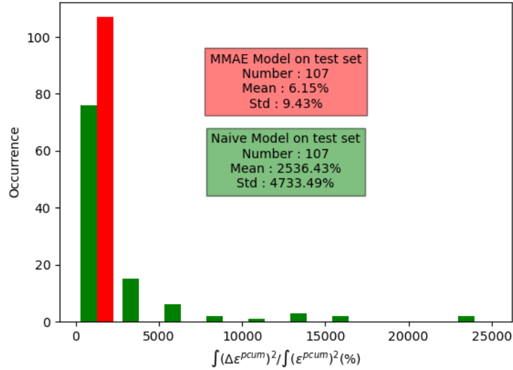
Figure 18: Histogram of the error for the test sets with the MMAE model and the naive model
