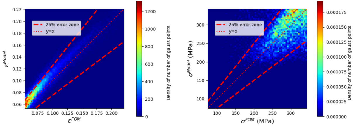
Figure 15: Error Graph on \epsilon^{pcum} and \sigma^{Mises} t=0.8 for defect 1042 from test dataset.
