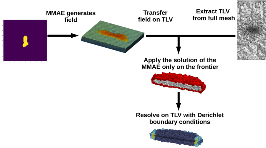
Figure 7: Online scheme
