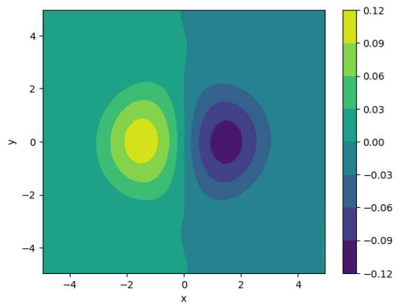
(f) Entropic Well-balanced scheme with 101 cells: u_y -velocity
