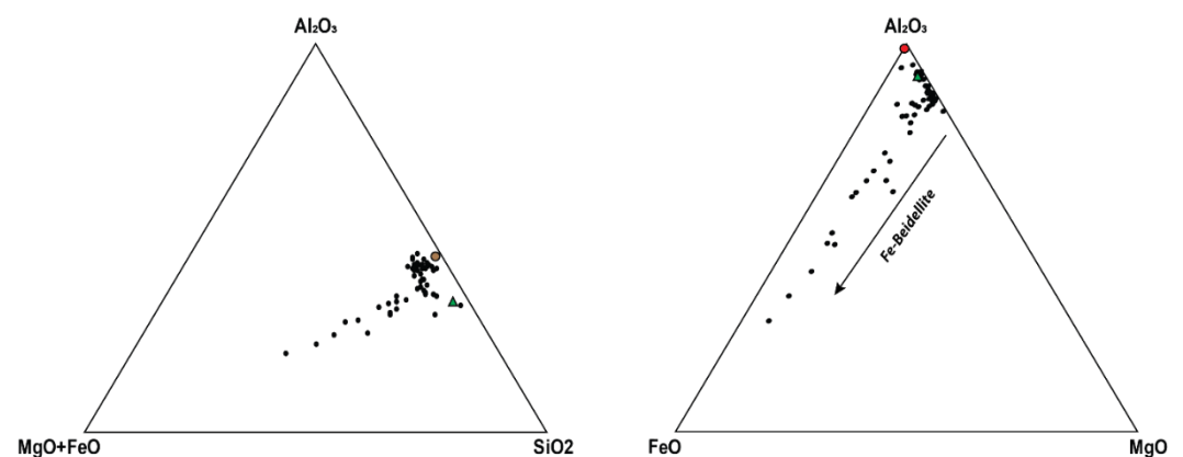
Figure 16. Ternary diagrams illustrating the distribution of clays within the samples. This distribution indicates iron enrichment of the clays toward a Fe-beidellite pole. Kaolinite (pink dot) and beidellite (green triangle) poles are also shown.
