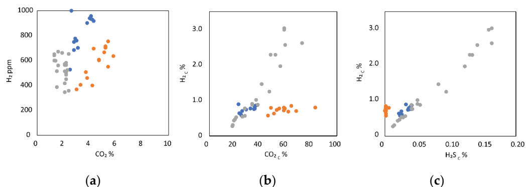
Figure 9. Diagram illustrating gas concentrations for the DJI-4 fumarole. (a) Non-corrected gas with H 2 in ppm versus CO 2 in %. (b) H 2 (%) versus CO 2 (%) after air correction. (c) H 2 (%) versus H 2 S (%) after air correction. Measurements were obtained on 21 November 2019 (orange dots), 12 August 2020 (blue dots), and 13 August 2020 (gray dots).
