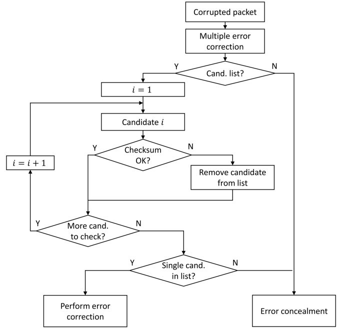
Fig. 4: Flowchart illustrating the correction process using both CRC and checksum to reduce the number of candidates in the output list
