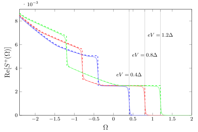
Fig. 2. Emission noise S^+(\Omega) (in units of e^2 \Delta ) as a function of frequency \Omega (in units of \Delta ) in the tunneling regime (transparency \tau = 0.02 ) and low temperature ( \theta = 0.01 \Delta ) for different values of the voltage bias. The full numerical result (full lines) is compared with the analytic form of Eqs. (15)-(18) (dashed lines).
