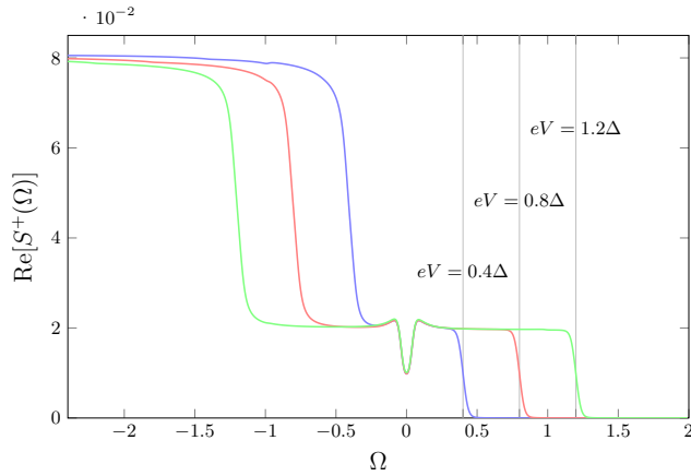
Fig. 4. Emission noise S^+(\Omega) (in units of e^2\Delta ) as a function of frequency \Omega (in units of \Delta ) for a symmetric N-dot-S junction, with coupling \Gamma = 0.02\Delta and low temperature ( \theta = 0.01\Delta ) for different values of the voltage bias.
