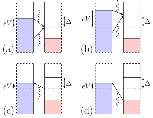
Fig. 3. Energy diagram of the junction illustrating emission [top part of (a) and (b)] and absorption [bottom part of (a) and (b), (c) and (d)] processes. Occupied electronic states are in light blue for the normal lead, and in light red for the TS one.
