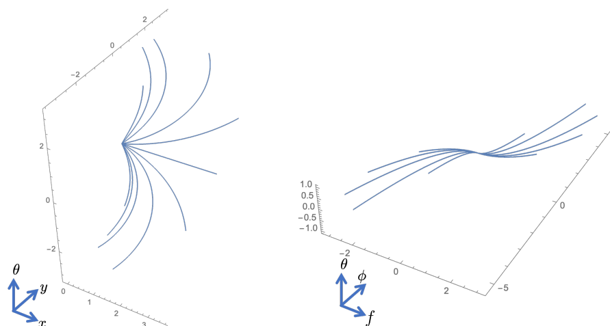
Figure 8. Horizontal integral curve fans corresponding to X_1 + c_2X_2 (left) and X_3 + c_4X_4 (right) where c_2 and c_4 are varied.
