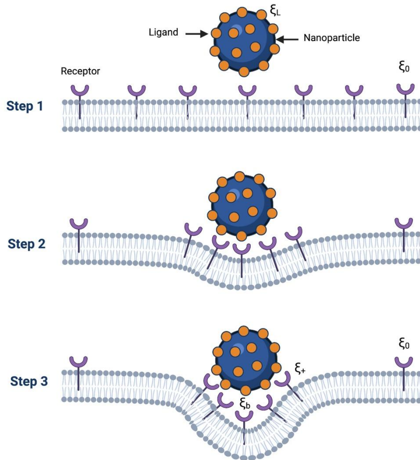
1 2 Figure 5: Schematic representation of the different steps for receptor-mediated wrapping of a 3 spherical nanoparticle. Step 1: Nonwrapped state. Step 2: binding state. Step 3: partially wrapped state. 4 \xi_0 is the receptor density in the remote region. \xi_+ is the receptor density in the depletion region. \xi_b is 5 the density of the receptor in the binding region. \xi_L is the ligand density on the nanoparticle surface.
