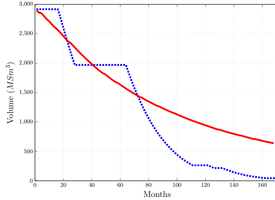
Figure 4: Evolution of the content of the reservoir in the one tank model. The dotted blue curve is the optimal trajectory of the amount of gas, while the red curve is the trajectory with the historical production
