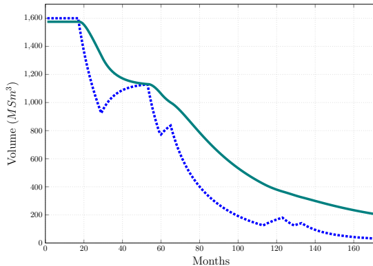
Figure 7: Evolution of the content of the reservoirs when applying the optimal policy in the two tanks model. The dotted blue curve shows the content of the first tank (linked to the well) while the green curve shows the content of the second tank
