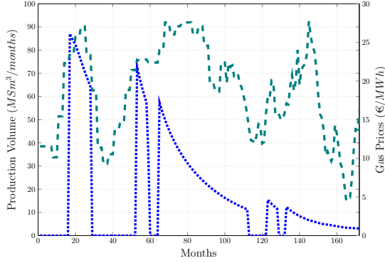
Figure 8: Trajectory of the optimal production in the two tanks model. The dotted blue curve is the optimal production, whereas the dashed green curve is the monthly gas price
