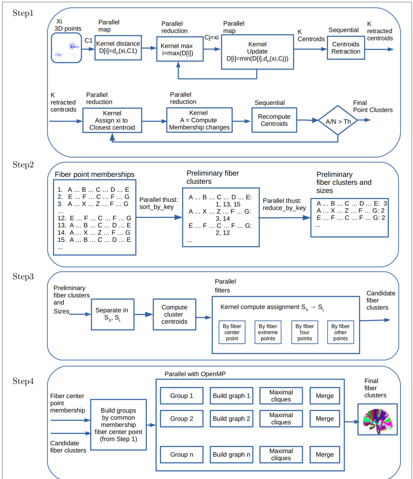
FIGURE 2 | Data flow and parallelism in GPU kernels. Step 1: Parallel point clustering, using Kmeans with point retraction computation with CUDA kernels based on parallel map and maximum and minimum reduction operations. Step 2: Building preliminary fiber clusters using parallel sort_by_key and reduce_by_key operations from thrust library. Step 3: Building candidate fiber clusters by reassignment of small to large preliminary clusters using point filters with CUDA kernels. Step 4: Building final fiber clusters with graph representation using OpenMP thread parallelism. Candidate clusters are separated in groups, where each group shares the fiber center point membership of Step 1, and then each thread creates and process a graph to produce the final clusters.
