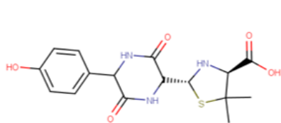
Amoxicillin diketopiperazine (AMX-DKP)
