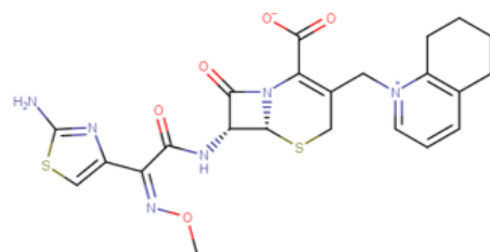
Cefquinome (CFQ)
