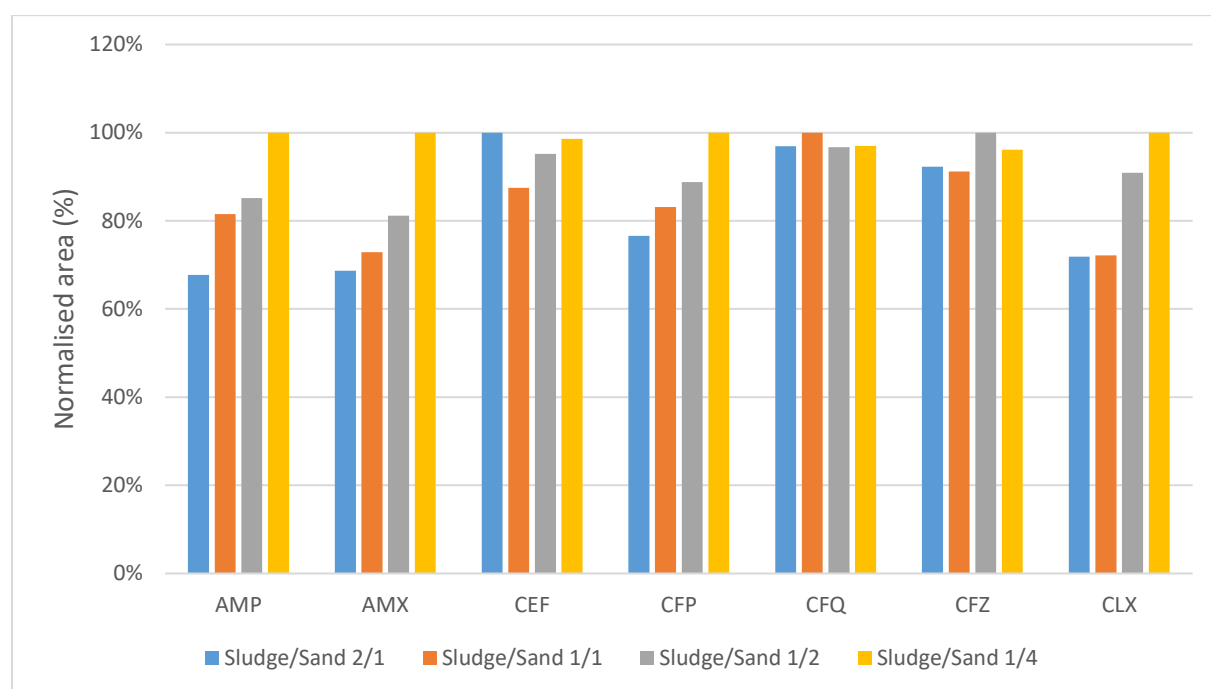
Figure 3 : Normalized area obtained for the extraction of the analytes with various sludge/sand ratio (500 mg sludge; extraction solvent: 5 mL H 2 O and 10 mL ACN).
