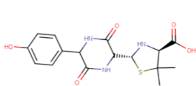
Amoxicillin diketopiperazine (AMX-DKP)
