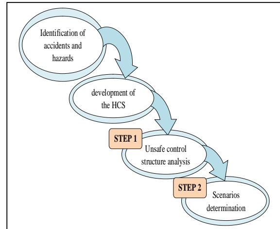
Fig. 2 STPA methodology
