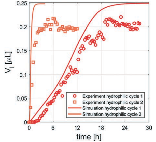
Fig. 9 The volume V_l of the salt solution in time for the 2D hydrophilic porous medium and pore network model for the first cycle (red) and second cycle (orange). In the second cycle, based after drying and recrystallization processes, multiple microcrystals are located close to the entrance which results in an 8 times faster deliquescence process compared to the first cycle.
