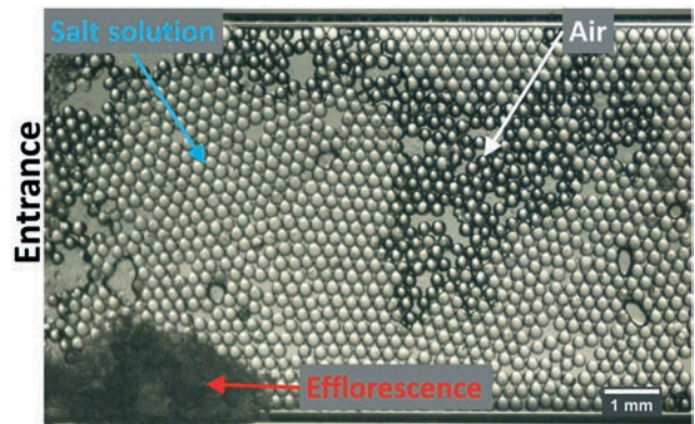
Fig. 11 Microscopy image of a multimodal pore size microporous medium. The porous medium is saturated with NaCl solution at saturation to monitor the drying. The air invasion is followed by subsequent crystallization of the NaCl.
