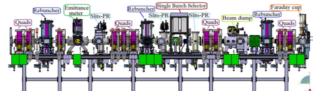
Figure 1: SPIRAL2 MEBT line layout.
