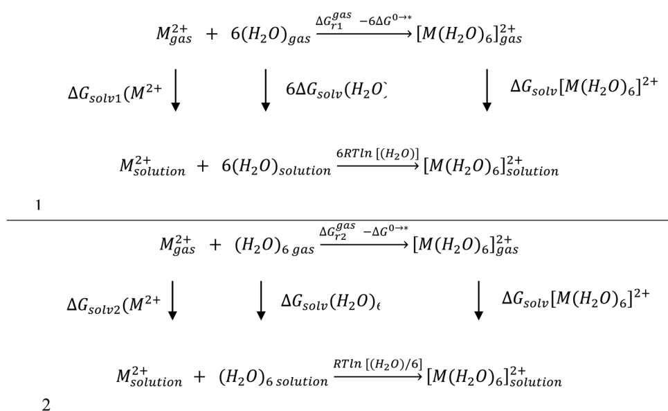
Fig. 1 The two thermodynamic cycles used for the hydration and complexation of the metal ion. Cycle 1 with 6H 2 O and cycle 2 with cluster of 6 water molecules.
