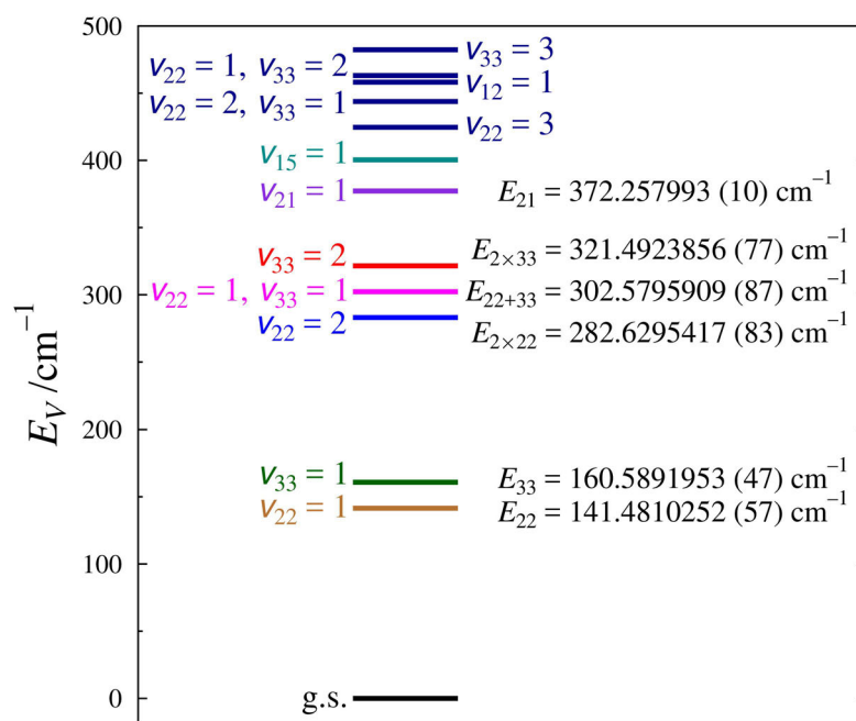
Fig. 2. The vibrational energy levels of benzonitrile below 500 \text{ cm}^{-1} , drawn from the anharmonic values of the CCSD(T)/ANO1 calculation. The denoted experimental energies result from the high-resolution infrared and perturbation analysis of the present work ( vide infra ). States colored in navy are not examined in this work; all states lower in energy are examined this work.
