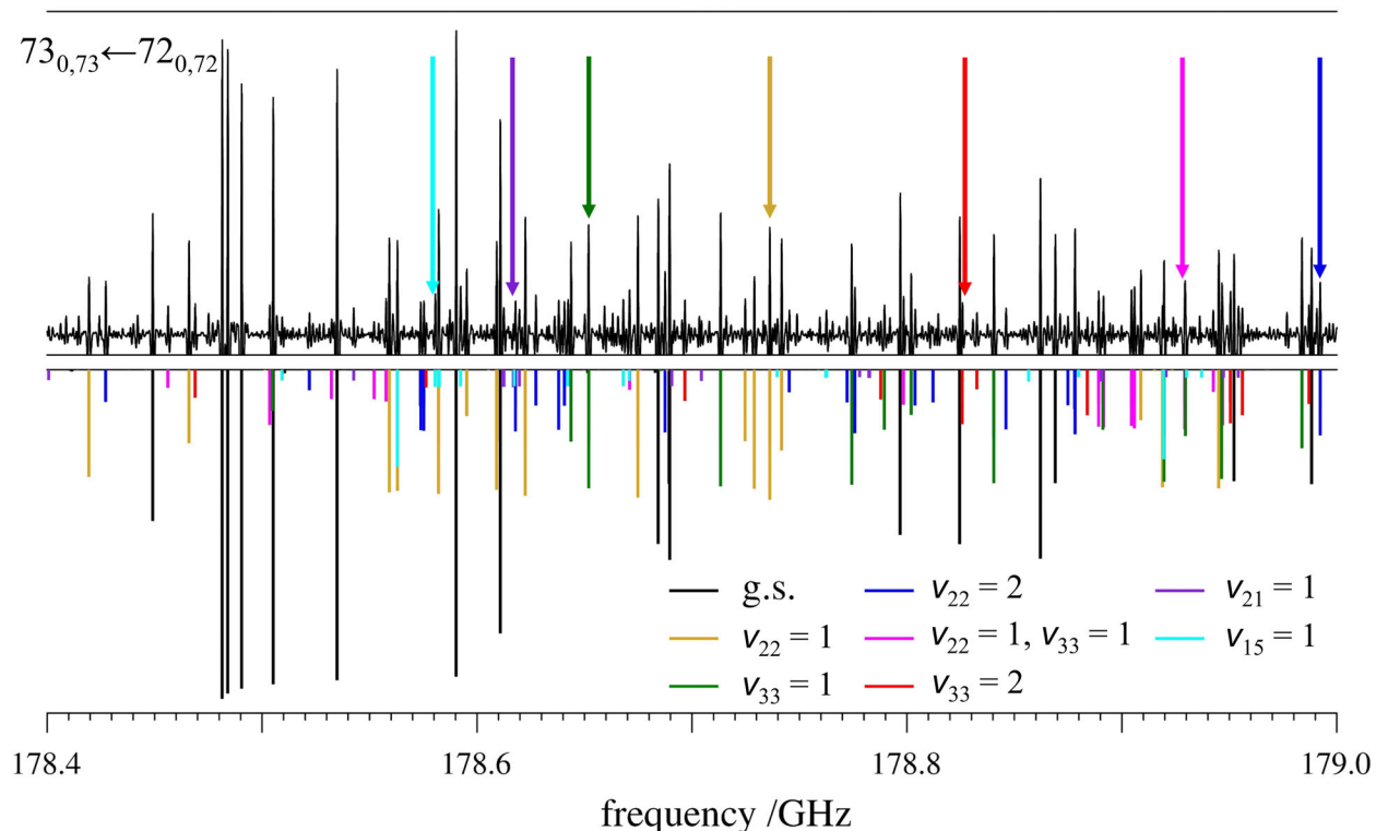
Fig. 4. Benzotrifluoride rotational spectrum from 178.4 to 179.0 GHz (top) and stick spectrum of the ground vibrational state and seven vibrationally excited states (bottom). The strongest transitions belong to the n = 2 , type-II + bands [66, 67]. The bandheads in this frequency region start at the 73_{0,73} \leftarrow 72_{0,72} transition of each vibrational state. The ground-state transition is near 178.48 GHz, and the corresponding transition for each excited state is marked with an arrow in the corresponding color. Numerous yet-to-be analyzed transitions belonging to other vibrational satellites are visible.
