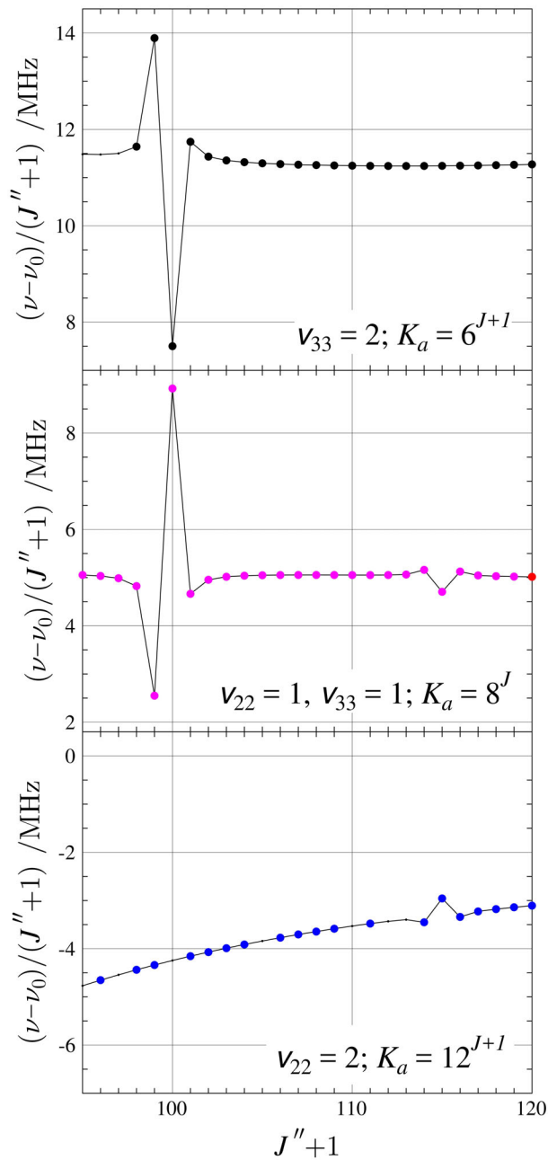
Fig. 10. Resonance plots depicting degenerate \Delta K_a = 2 and \Delta K_a = 4 local perturbations between v_{22} = 2 and v_{22} = 1, v_{33} = 1 at J'' + 1 = 115 and between v_{22} = 1, v_{33} = 1 and v_{33} = 2 at J'' + 1 = 99, 100 . At J'' + 1 = 115 , the v_{22} = 2, K_a = 12^{J+1} series is degenerate with K_a = 11^J . In the depicted J'' + 1 range, the v_{22} = 1, v_{33} = 1 series is degenerate K_a = 8^J, 9^{J+1} , and the v_{33} = 2 series is degenerate K_a = 5^J, 6^{J+1} . Measured transitions are represented by circles and predictions from the final coupled fit are black lines. Red circles indicate transitions with |(f_{\text{obs.}} - f_{\text{calc.}})/\delta f| \geq 3 . The three plots have identical scaling along the vertical axis, and the respective exact mirror image correspondence confirms the K_a assignment of the resonance partners.
