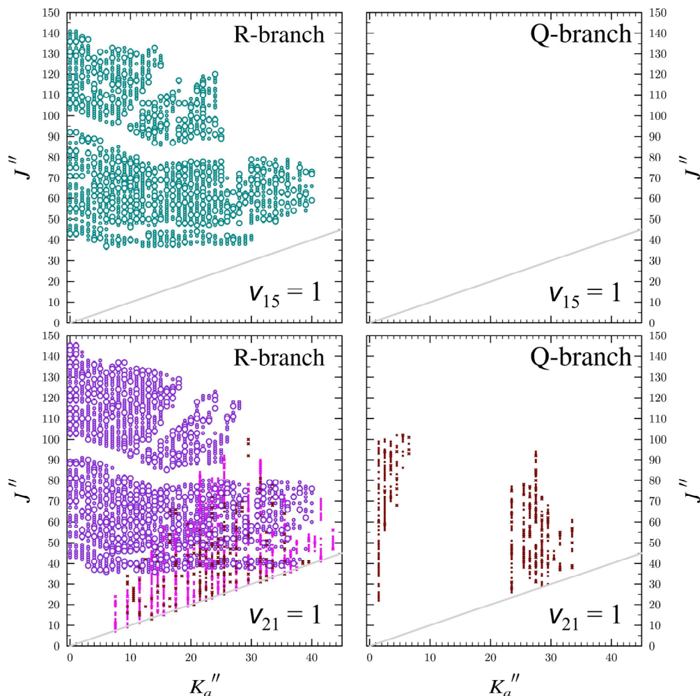
Fig. 12. Data distribution plots for \nu_{21} = 1 (bottom) and \nu_{15} = 1 (top) of benzotrile. The size of the plotted symbol is proportional to the value of |(f_{\text{obs.}} - f_{\text{calc.}})/\delta f| , where \delta f is frequency measurement uncertainty, and all values are smaller than 3. Circles denote millimeter-wave data. Colored crosses mark infrared data from the ground vibrational state to \nu_{21} = 1 (magenta color indicates R-branch transitions), and are shifted up by 0.5 along the K_a axis for viewing convenience. The \nu_{15} mode is not infrared active.
