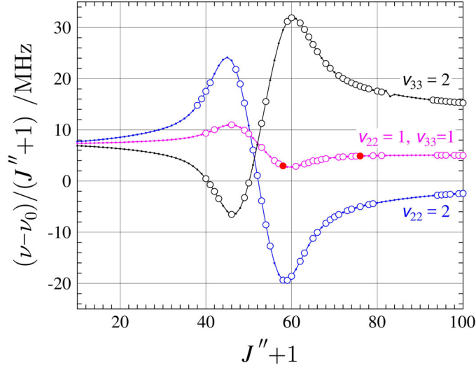
Fig. 9. Difference frequency plot for K_a = 9^J rotational transition sequences in \nu_{22} = 2 (blue), \nu_{22} = 1 , \nu_{33} = 1 (magenta) and \nu_{33} = 2 (black) vibrational states, indicating the effect of distortion and perturbation among the three states. The plotted values are frequency differences between excited state transitions and their ground-state counterparts, scaled by (J''+1) in order to make the plots more horizontal. Measured transitions are represented by open circles, while red circles indicate measurements with |(f_{\text{obs.}} - f_{\text{calc.}})/\delta f| \geq 3 . A resonance is visible near J'' + 1 = 84 for \nu_{33} = 2 .
