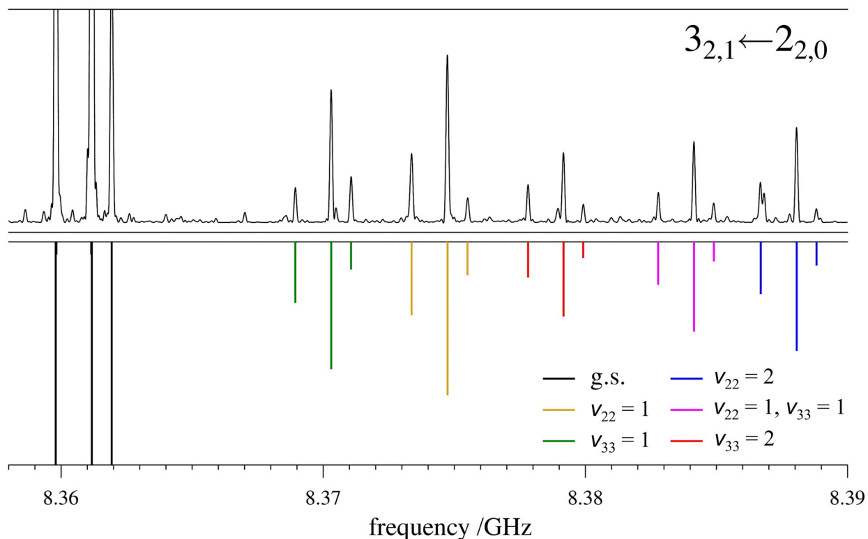
Fig. 13. Benzotrile rotational spectrum from 8.358 to 8.390 GHz (top) and stick spectrum of the ground vibrational state and five vibrationally excited states (bottom). The transitions in this frequency region are hyperfine-resolved 3_{2,1} \leftarrow 2_{2,0} rotational transition of each vibrational state.
