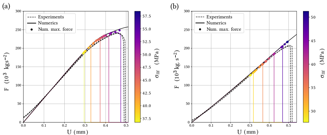
Figure 10: (a) Experimental force and numerical maximum force vs displacement for D = -0.4 mm (b) Experimental force and numerical maximum force vs displacement for D = -2.5 mm.
