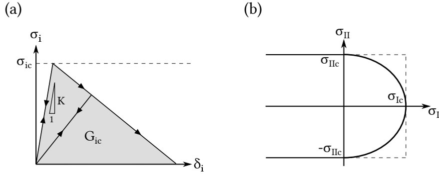
Figure 3: (a) Bilinear traction-separation relation in mode i and (b) Critical stress mixity relation
