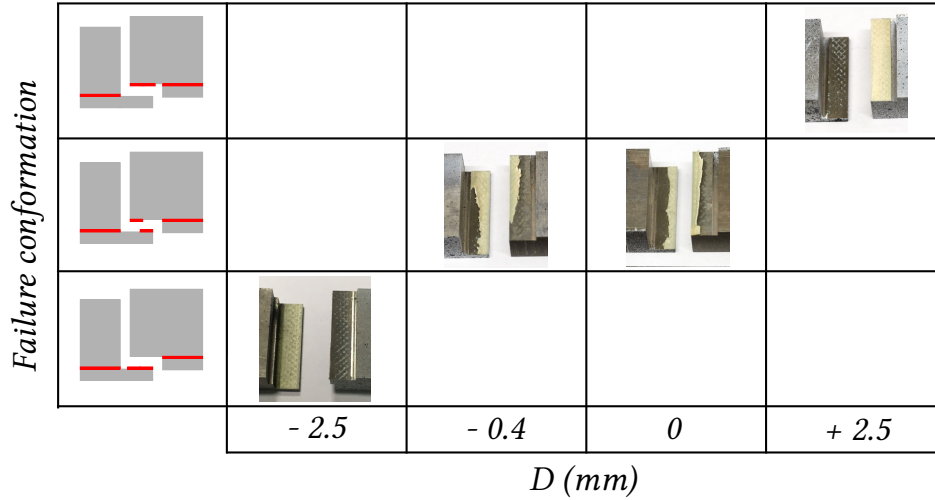
Figure 7: Failure conformation as a function of the shift parameter D
