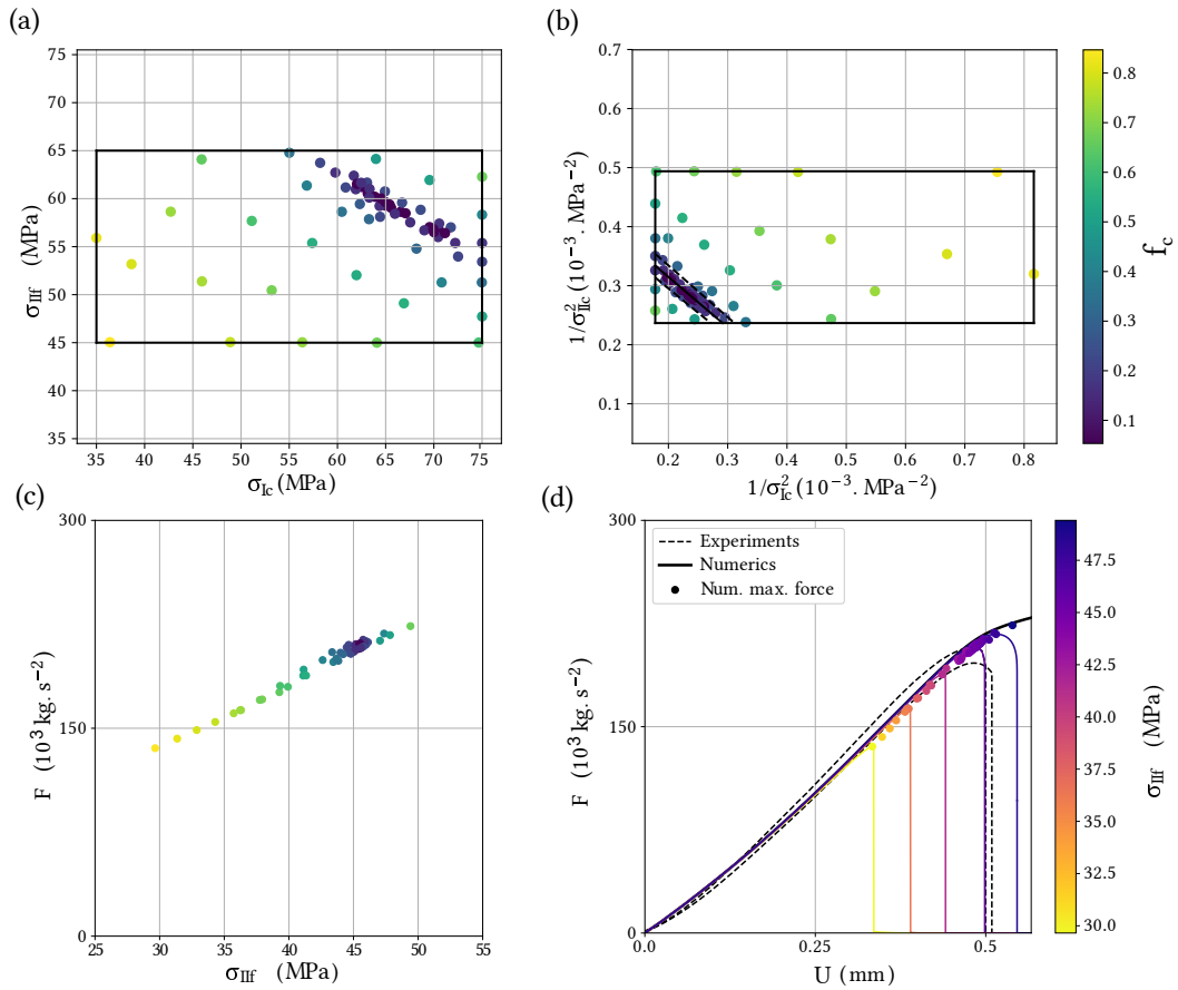
Figure 9: For D = +2.5 mm: (a) Cost function versus \sigma_{Ic} and \sigma_{IIc} , (b) Cost function versus 1/\sigma_{Ic}^2 and 1/\sigma_{IIc}^2 , (c) Numerical maximum force F as a function of \sigma_{IIc} (d) Experimental force and numerical maximum force vs displacement. The colorbar displayed on figure (b) is shared with (a) and (c).
