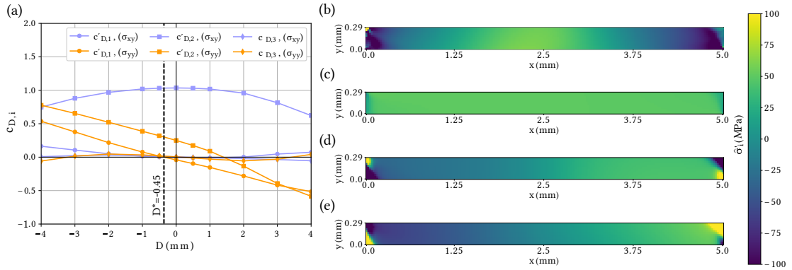
Figure 6: With the elasto-visco-plastic model: (a) Projections on the three main eigen modes, where c'_{D,i} is the projection of \sigma_i on \hat{\sigma}'_i and c'_{D,3} the projection of \sigma_i on \hat{\sigma}_3 (b) \sigma_{xy} first mode, (c) \sigma_{xy} second mode, (d) \sigma_{yy} first mode, (e) \sigma_{yy} second mode
