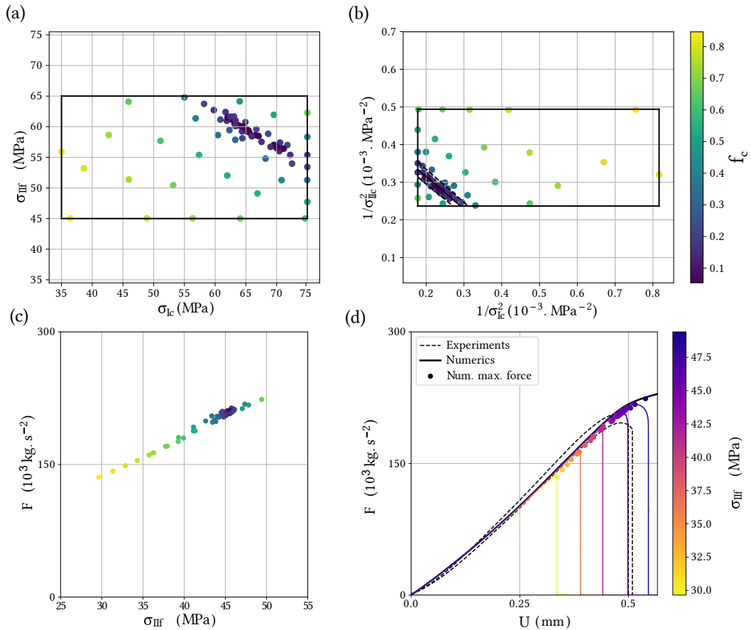
Figure 9: For D = +2.5 mm: (a) Cost function versus \sigma_{Ic} and \sigma_{IIc} , (b) Cost function versus 1/\sigma_{Ic}^2 and 1/\sigma_{IIc}^2 , (c) Numerical maximum force F as a function of \sigma_{IIc} (d) Experimental force and numerical maximum force vs displacement. The colorbar displayed on figure (b) is shared with (a) and (c).
