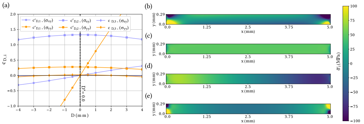
Figure 12: With the elastic model and a geometry such as described in the standard ISO 11003: (a) Projections on the three main eigen modes, where c'_{D,i} is the projection of \sigma_i on \hat{\sigma}'_i and c'_{D,3} the projection of \sigma_i on \hat{\sigma}_3 (b) \sigma_{xy} first mode, (c) \sigma_{xy} second mode, (d) \sigma_{yy} first mode, (e) \sigma_{yy} second mode
