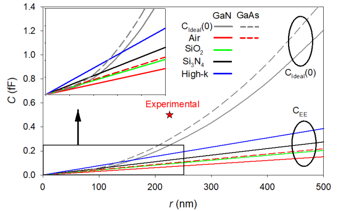
Fig. 6. C_{\text{ideal}}^T(0) and C_{\text{EE}}^T (for different dielectric materials) as a function of the radius r of the anode in the reference diode of Fig. 1 considered to be circular. The dashed lines correspond to GaAs, and the point is the experimental value for the total capacitance of the THz SBD of Maestrini et al. [23]. The inset shows a zoomed-in view of r from 0 to 250 nm.
