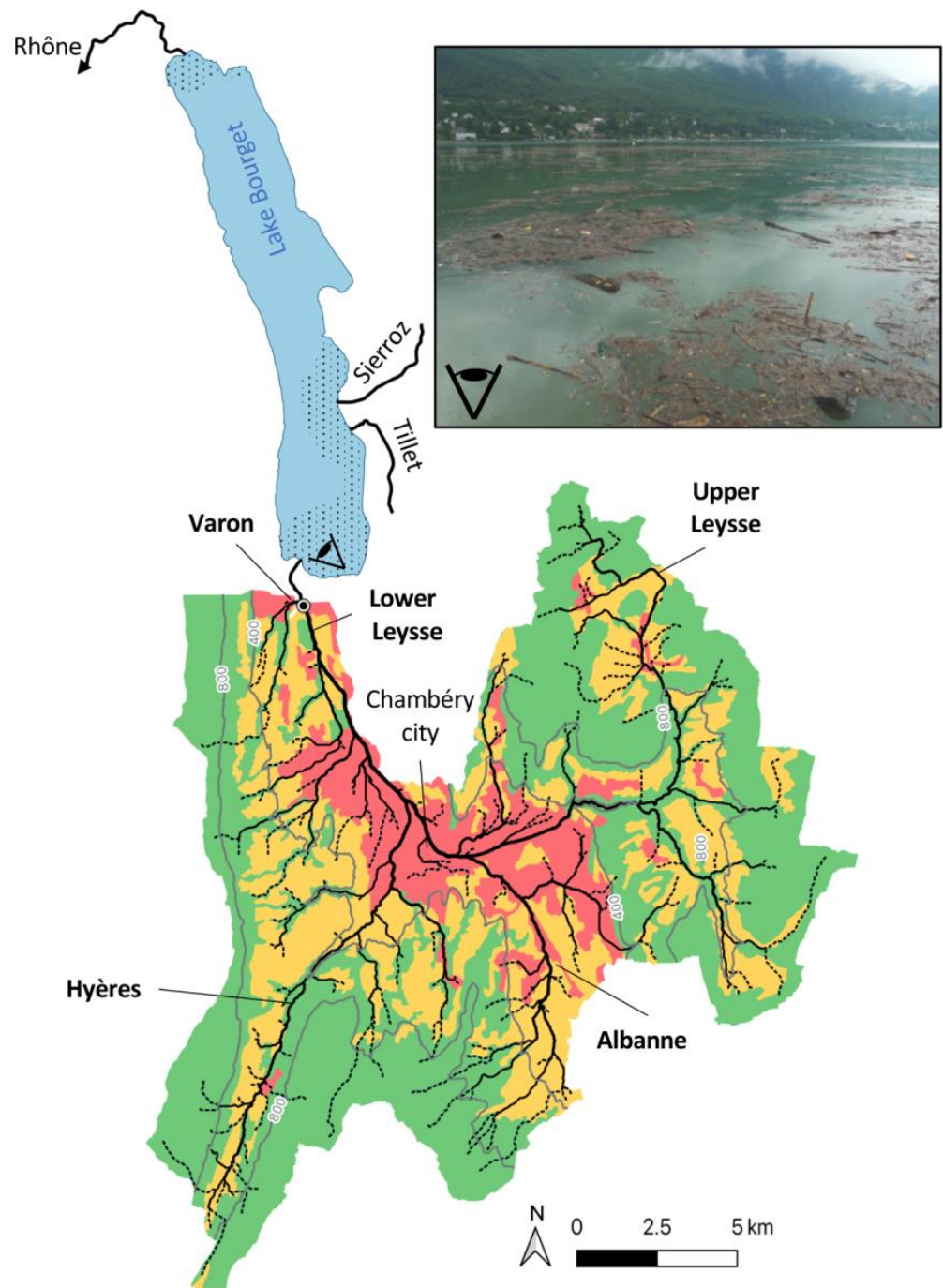
Figure 1. Map of the Leysse River catchment. Land uses are shown following Corine Land Cover (green: forest; yellow: agriculture; red: urban). The elevation contour lines 400 m and 800 m are shown in gray. Rivers are indicated in black, intermittent creeks being in dotted lines. The black dot indicates the university bridge where CPOM measurements were made. The dotted area in Lake Bourget indicates the presence of gas bubbles in the sediment [32]. The photograph showing floating litter on the lake was taken after a large flood.
