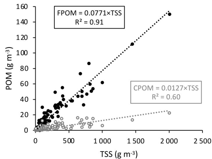
Figure 4. Instantaneous transport of CPOM (grey open dots) and FPOM (black dots) ( \text{g m}^{-3} ) in relation to TSS ( \text{g m}^{-3} ).
