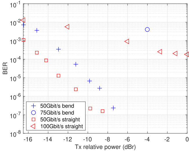
Fig. 19. BER versus Tx relative power for straight 10 mm and 10-bend using I-Q modulation.
