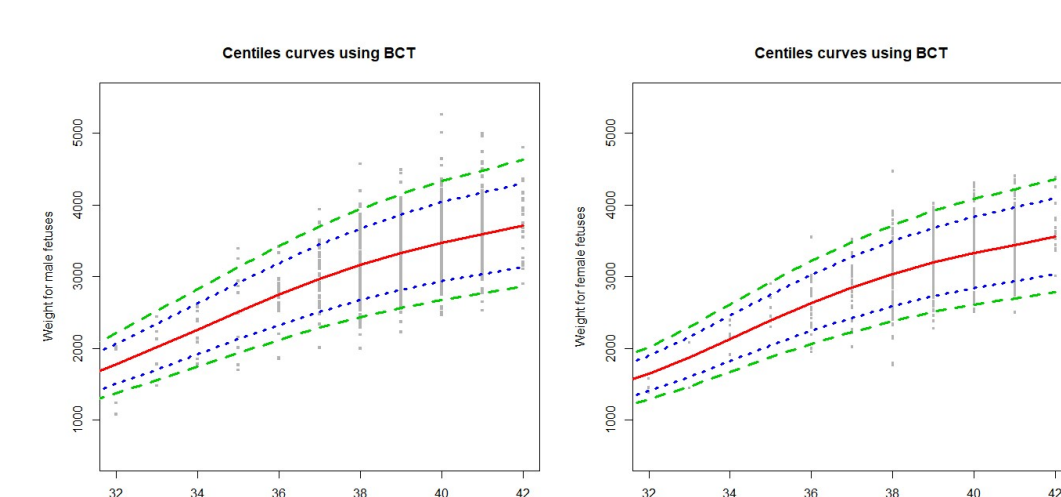
Figure 5: Centiles curves using the Box-Cox t (BCT) distribution for the male and female fetuses weight data and cubic splines smoothing.
