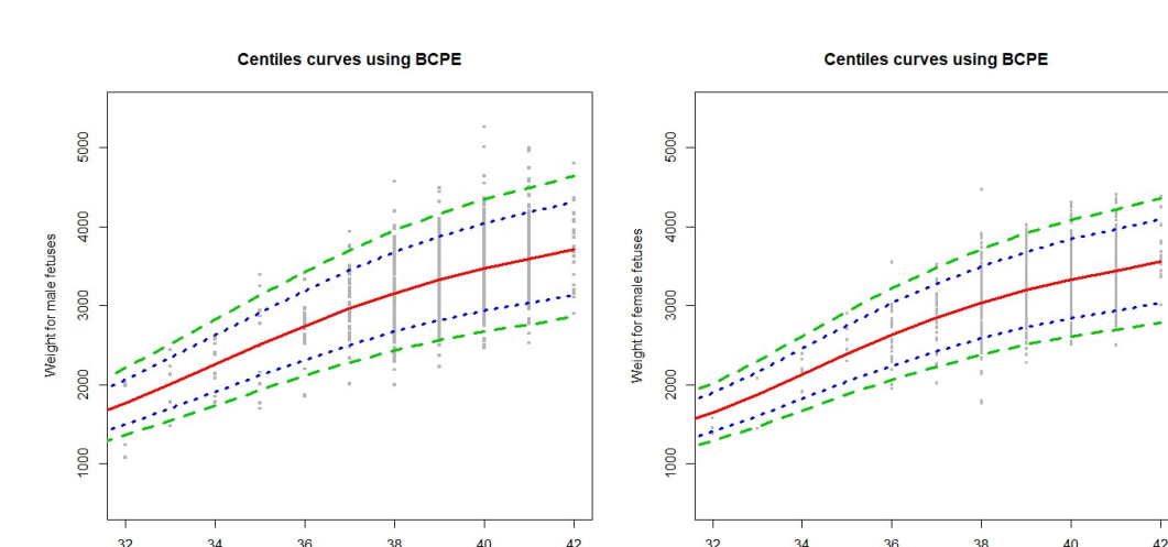
Figure 4: Centiles curves using the Box-Cox power exponential (BCPE) distribution for the male and female fetuses weight data and cubic splines smoothing.
