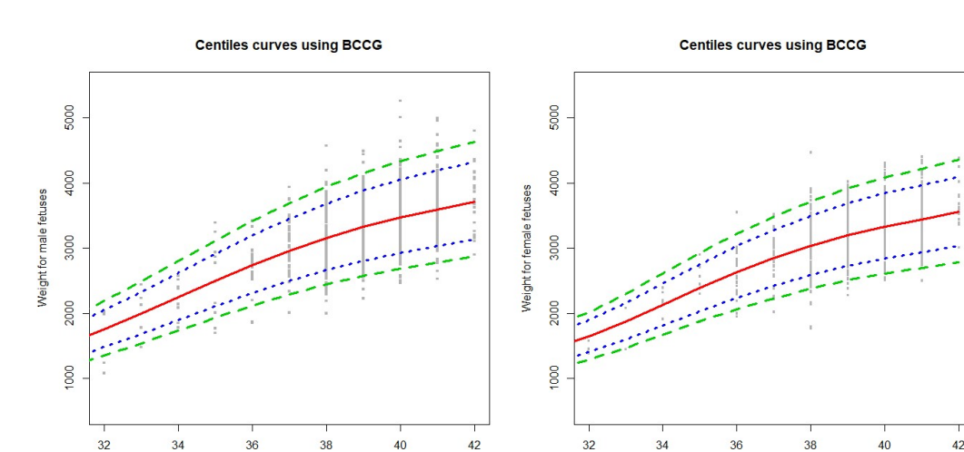
Figure 3: Centiles curves using the Box-Cox and Green (BCCG) distribution for the male and female fetuses weight data and cubic splines smoothing.
