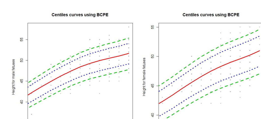
Figure 7: Centiles curves using the Box-Cox power exponential (BCPE) distribution for the male and female fetuses height data and cubic splines smoothing.
