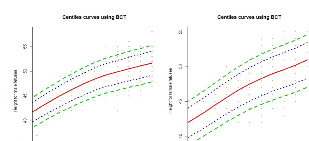
Figure 8: Centiles curves using the Box-Cox t (BCT) distribution for the male and female fetuses height data and cubic splines smoothing.
