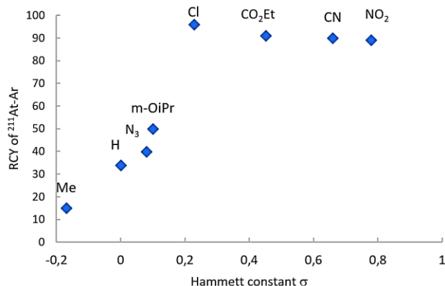
Figure 3. RCY of ^{211}At -labeling of arylidonium ylides using method A for 30 min in function of their Hammett constant.
