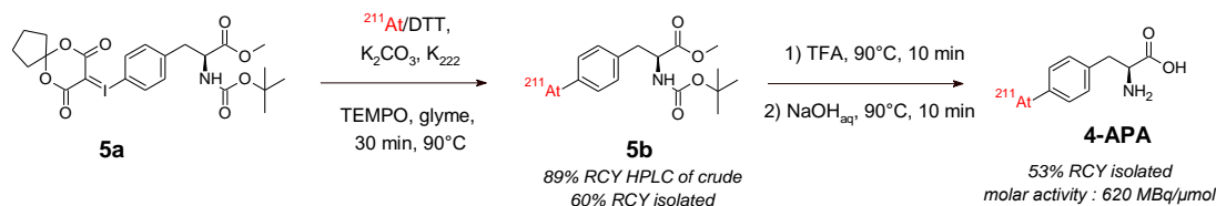
Scheme 3. Preparation of 4-[ 211 At]astatophenylalanine from precursor 5a
