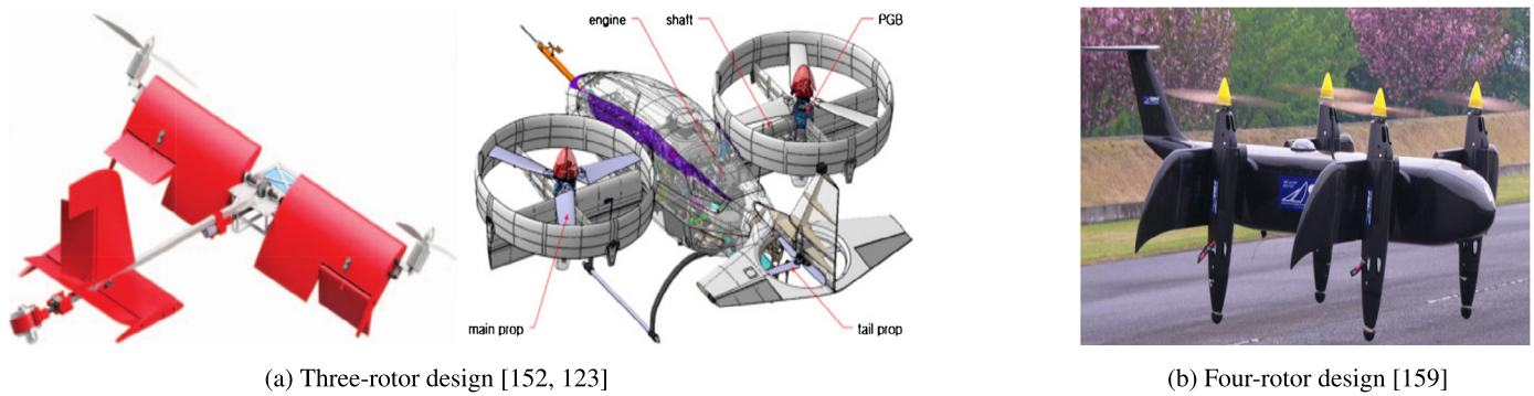
Fig. 4. Examples of tilting UAVs.
