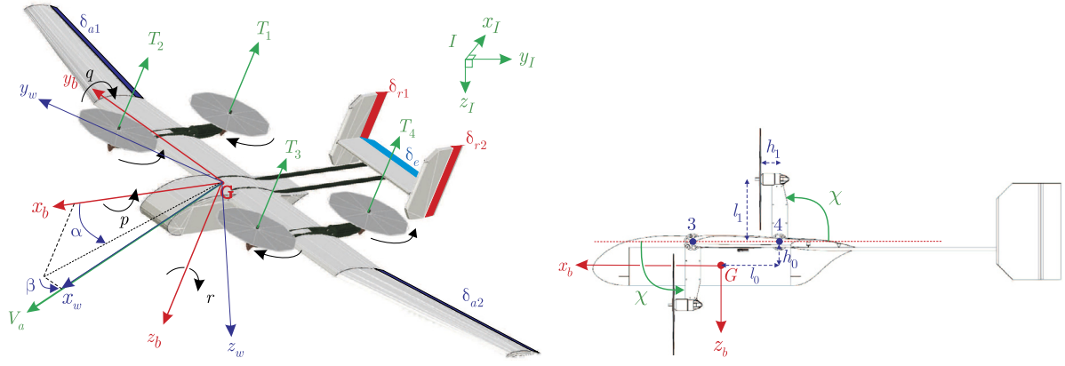
Fig. 6. Left: tiltrotor in helicopter mode, propellers tilted by \chi = 0 [rad]. Right: fixed-wing mode, propellers tilted by \chi = \frac{\pi}{2} [rad] [134].
