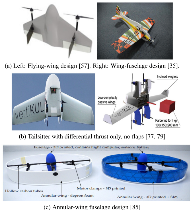
Fig. 2. Examples of tailsitter UAVs.
