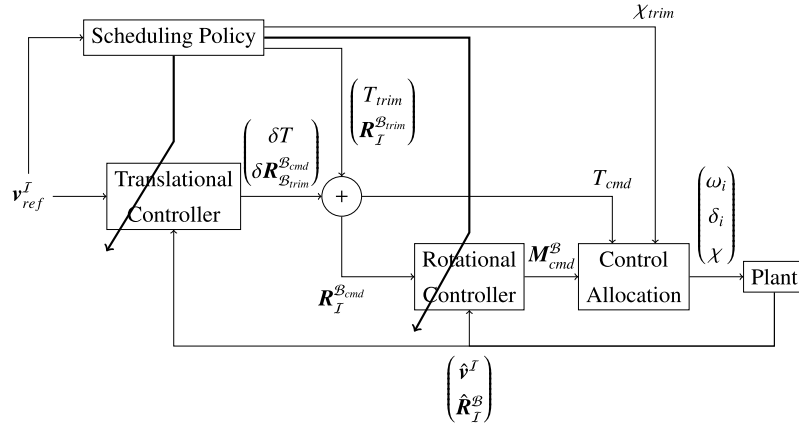
Fig. 13. Scheduled control approach: Given a desired velocity reference v_{ref}^I , the scheduling policy loads the translational and rotational controller of the corresponding linearization point. The associated trim values for the thrust T_{trim} and attitude R_I^{B_{trim}} are then combined with the controller commands, namely the thrust \delta T and the thrust vector alignment attitude \delta R_I^{B_{cmd}} . Control torques M_{cmd}^B from the rotational controller are fed into the control allocation, together with the total thrust T_{cmd} and the trim tilt angle \chi_{trim} (only for tiltrotor and tilting vehicles) to compute the actuator commands for the hybrid UAV.
