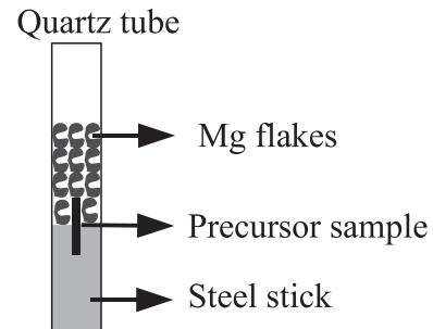
Appendix 1. Illustration of experimental set-up.
