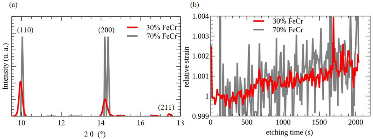
Fig. 5. (a) XRD diffraction pattern after chemical etching ( t = 1700\text{s} ) (b) Evolution of the relative lattice parameter during the Mg phase etching of 30%FeCr (red) and 70%FeCr samples (gray).
