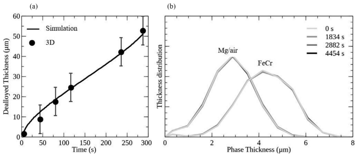
Appendix 3. (a) Evolution of dealloying thickness with time from (\text{FeCr})_{70}\text{Ni}_{30} precursor sample. To be able to compare simulation and experimental values, the experimental incubation time was subtracted from the experimental time. The continuous line corresponds to the simulation. (b) Evolution of FeCr and Mg/air phase thickness during sacrificial phase etching step of a dealloyed sample from a (\text{FeCr})_{70}\text{Ni}_{30} precursor.
