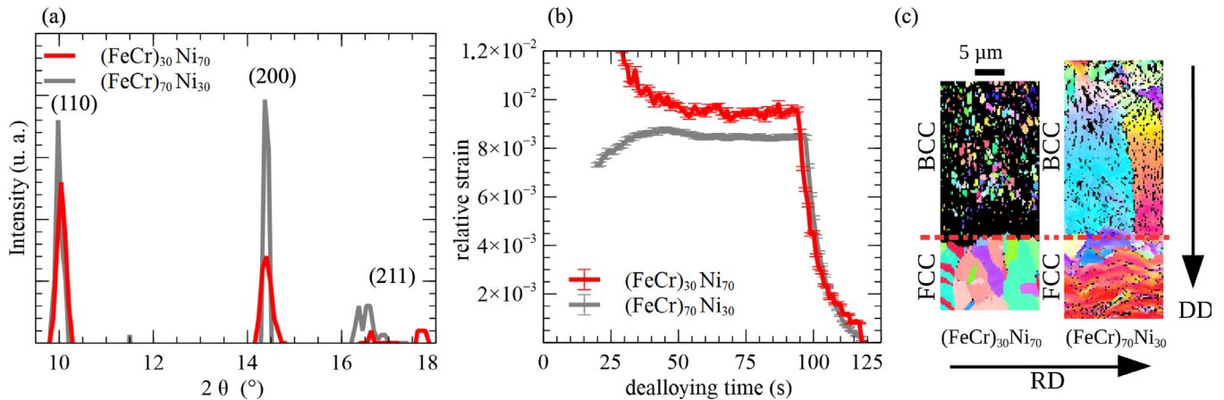
Fig. 6. (a) XRD diffraction pattern of the BCC phase ( t = 80\text{ s} ) (b) Evolution of relative strain and of BCC dealloyed diffraction peaks (111) during dealloying of a (\text{FeCr})_{30}\text{Ni}_{70} (red) and (\text{FeCr})_{70}\text{Ni}_{30} (gray) precursors (c) IQ+IPF SEM-EBSD map after 3 mins dealloying at 933 K from (\text{FeCr})_{30}\text{Ni}_{70} (left) and (\text{FeCr})_{70}\text{Ni}_{30} (right). The bottom part corresponds to the precursor and the top part to dealloyed portion. Arrows correspond to the cold-rolling direction (RD) and dealloying reaction direction (DD).
