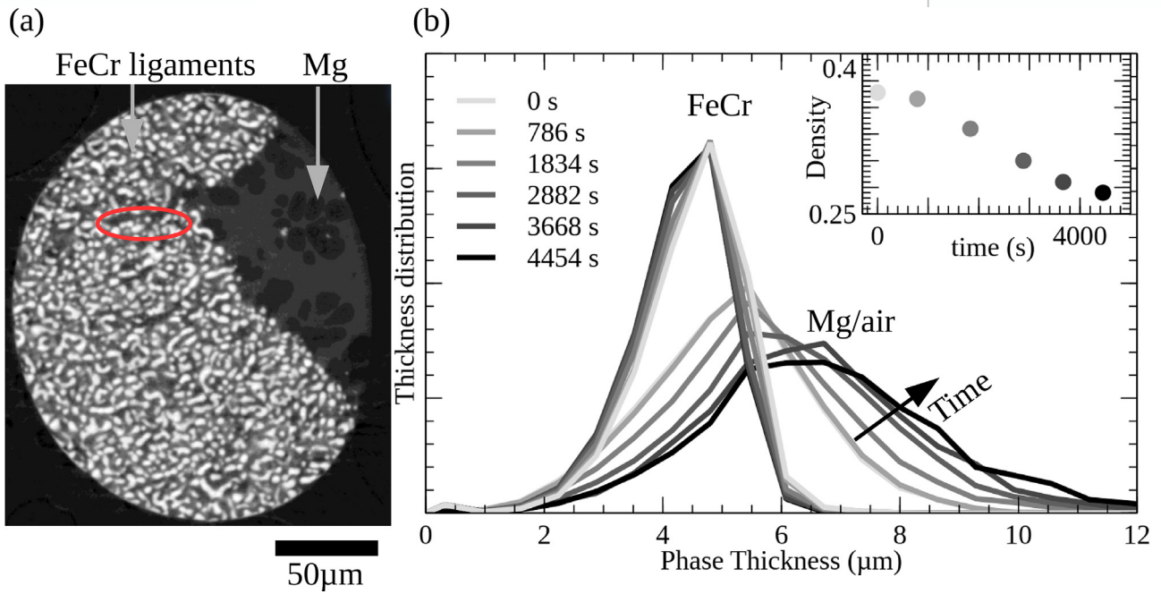
Fig. 4. (a) 2D view extracted from a 3D reconstruction for t = 1048 s. The red ellipse highlights a defect (b) Evolution of FeCr and Mg/air-etchant phase thickness during the sacrificial phase etching step. As inset, the evolution of the FeCr phase volume ratio (relative density) is plotted.
