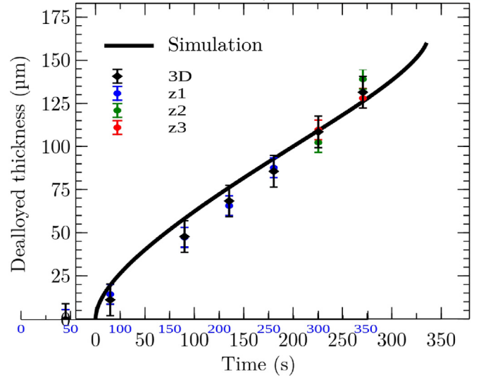
Fig. 2. Evolution of dealloying thickness with time for 2D and 3D measurements (blue axis). The continuous line corresponds to the simulation (black axis).
