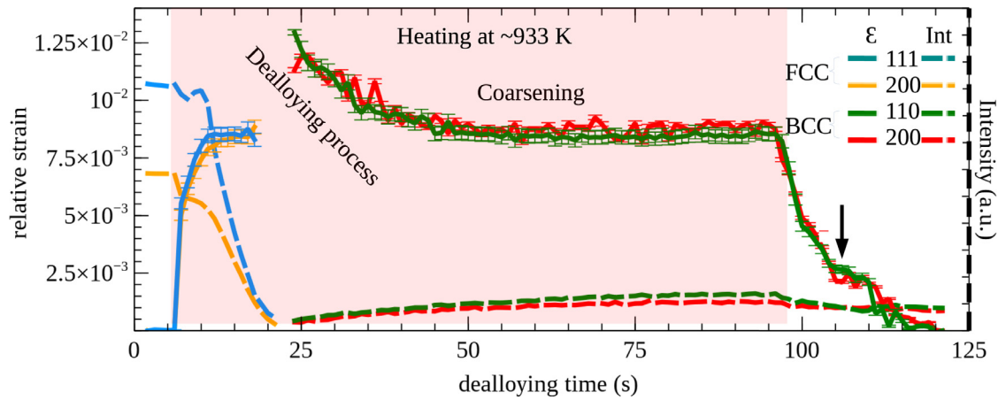
Fig. 3. Evolution of relative strain (continuous lines) and intensity (dashed lines) of 2 different FCC precursors and 2 different BCC dealloyed diffraction peaks during dealloying. The arrows highlight interaction between the 2 phases during the cooling step.
