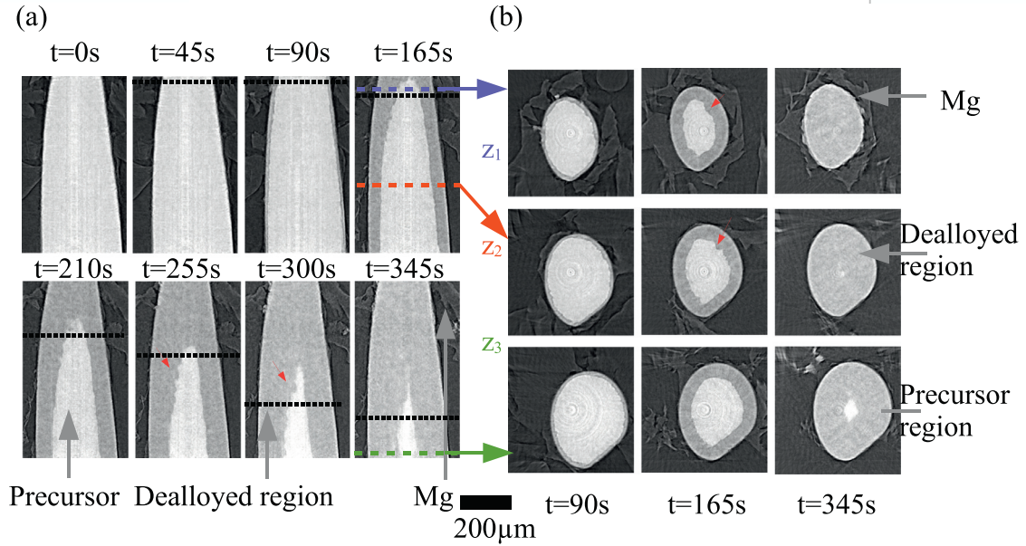
Fig. 1. Evolution of a dealloying front during the dealloying process from (FeCr)30Ni70 (a) sagittal slices of the sample at different intervals (b) 3 different horizontal slices at 3 intervals corresponding approximately to the position of the dashed colored lines in (a). Black dashed lines correspond to the volume used to quantify the evolution of the dealloying process. Red arrows highlighted some irregularities noticed at the precursor/dealloying part boundaries.
