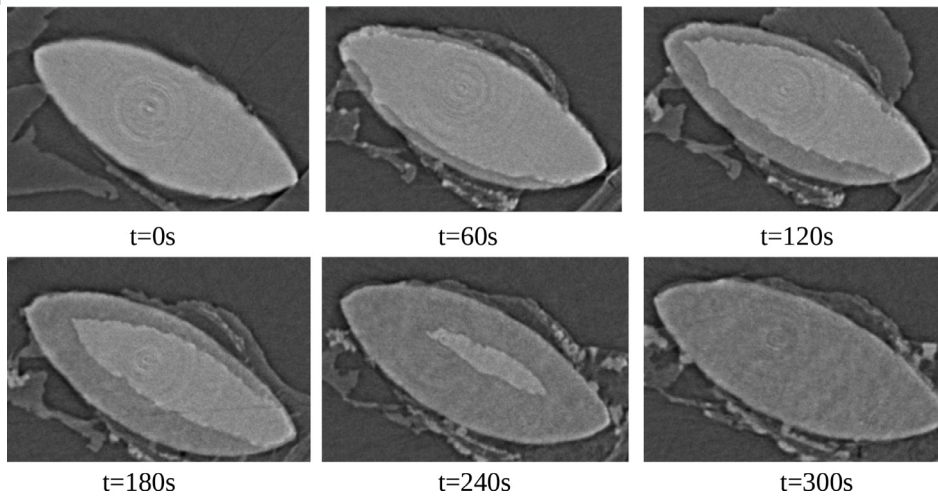
Appendix 2. Sagittal slices extracted from the 3D reconstruction showing the evolution of dealloying front during dealloying process from (\text{FeCr})_{70}\text{Ni}_{30} precursor sample. Light gray and median gray correspond respectively to precursor area and to dealloyed area.
