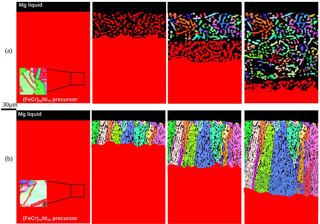
Fig. 7. Grain formation during dealloying. The red part corresponds to the FCC phase. (a) for a low amount of FeCr, the high kinetics of dealloying promotes a morphological transformation with the formation of FCC ligaments followed by a displacive transformation, (b) for a high amount of FeCr, the slow kinetics of dealloying promotes a diffusive transformation with the direct formation of BCC ligaments.
