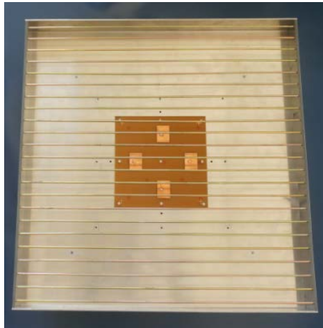
Figure 6. Realized prototype of the FP OAM antenna.
