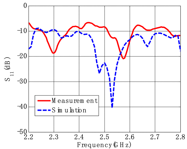
Figure 7. Simulated and measured reflection coefficients of the FP OAM antenna.
