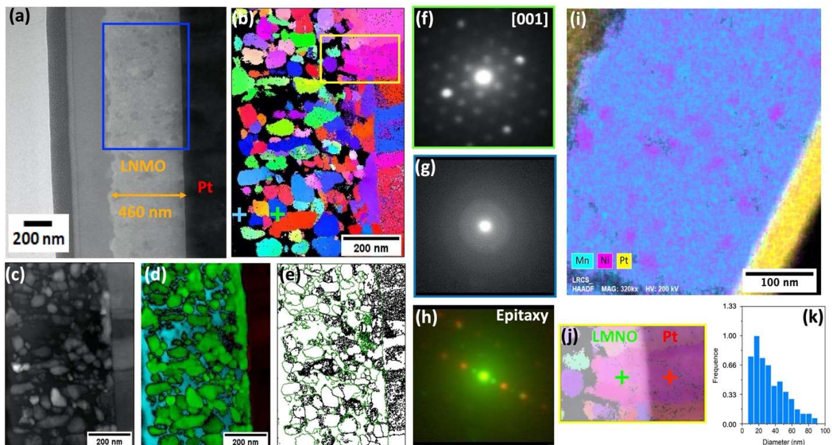
Figure 4: (a) TEM image of the LMNO FIB lamella sample before cycling, (b) orientation map according to the Y axis, (c) index map (d) phase map where black represents the platinum, in green the LMNO phase and in blue the amorphous phase; (e) grain boundaries map, (f-g-h) electron diffraction pattern of spinel LMNO, porosity and combination of platinum and LMNO showing the epitaxial effect between the two phases, (i) EDS mapping showing Si in black, Pt in yellow, pink and blue corresponds to Mn and Ni respectively, (j) epitaxial effect of LMNO on Platinum (k) Grain size distribution map of the analyzed area.
