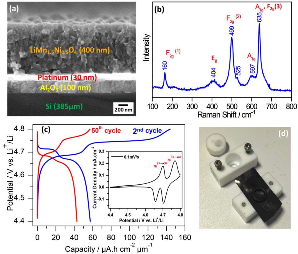
Figure 1. Structural and electrochemical characterization of the pristine LMNO thin film. (a) SEM image of cross section of the LMNO/Si/ \text{Al}_2\text{O}_3 /Pt stacking after annealing at 700°C during 2h in air. (b) Raman spectrum of the LMNO thin film. (c) 2 nd and 50 th charge-discharge cycles of the LMNO thin film recorded at 1C rate (147 \text{mA}\cdot\text{g}^{-1} ) in a conventional electrochemical flat cell. In insert: cyclic voltammetric curves recorded at 0.1 mV/s. (d) Electrochemical flat cell used for electrochemical cycling of LMNO thin film. 1M \text{LiClO}_4 EC:DMC 1:1 electrolyte.
