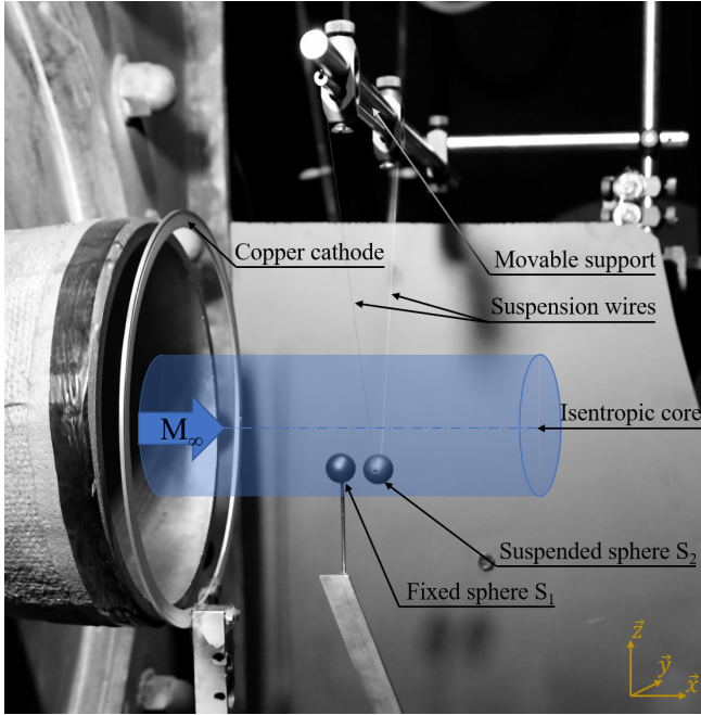
Figure 3: Picture of the swinging sphere set-up
